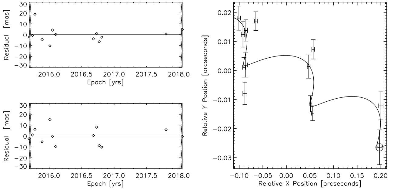
Fig. A.1. Left panels: residuals in mas as a function of epoch for right ascension ( bottom ) and declination ( top ). Right panel: solution for the parallax determination. We show the results for CFHT-Hy-20, the results for CFHT-Hy-21 are displayed in Fig. 3. The circle dot marks the reference epoch.
