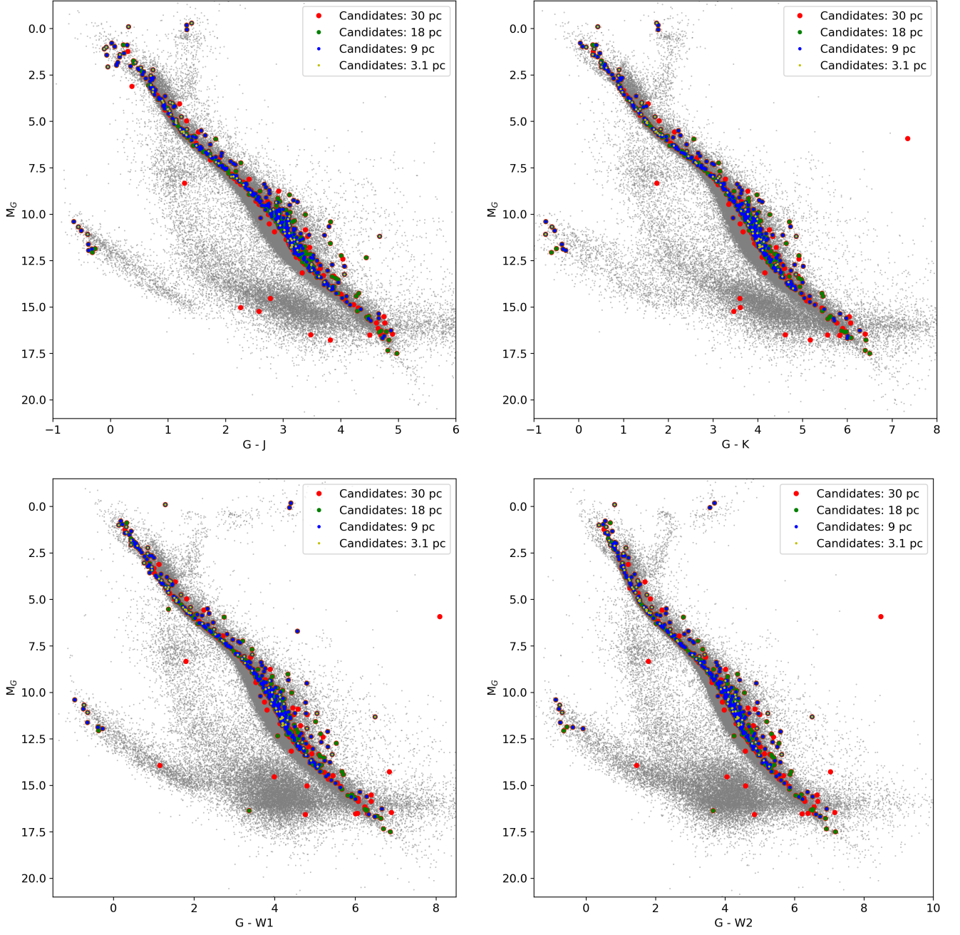
Fig. B.2. Colour–magnitude diagrams combining the Gaia magnitude with infrared photometry from 2MASS ( J + K_s ) and AllWISE ( W1 + W2 ). Symbols are as in Fig. B.1.
