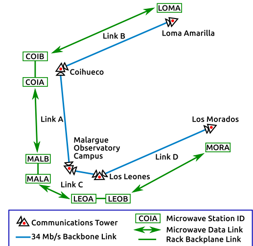
Fig. 13. Configuration of the high capacity microwave backbone network that connects the four FD sites with the main campus control and data acquisition center in Malargüe.
