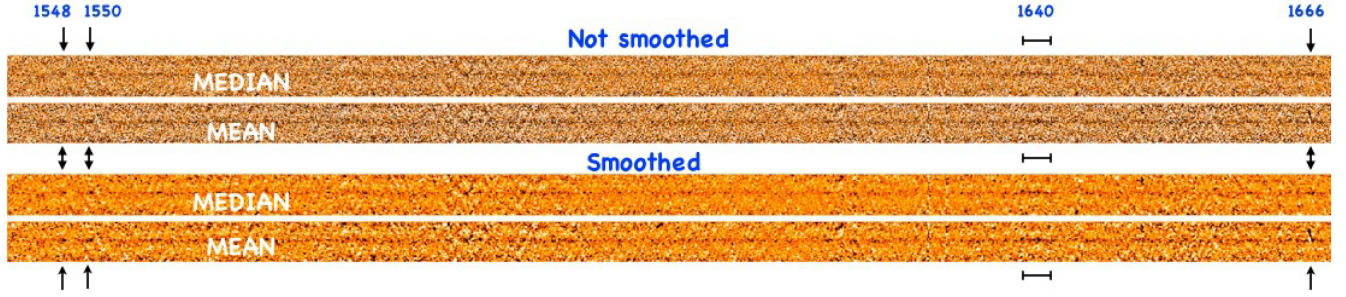
Figure 4. The two-dimensional X-Shooter spectrum of Ion2 reporting the faint continuum and the C IV \lambda\lambda 1548, 1550 , He II \lambda 1640 , and O III \lambda\lambda 1661, 1666 emission lines is shown (indicated with arrows and a segment for the He II \lambda 1640 emission). This figure shows the different broadness of the lines: the width of the segment is \sim 500 \text{ km s}^{-1} , whereas the other C IV \lambda\lambda 1548, 1550 and O III \lambda\lambda 1661, 1666 lines are much narrower and possibly not resolved ( \sigma_v < 25 \text{ km s}^{-1} ). The top panels show the non-smoothed mean and median spectra. The same is reported in the bottom panels after applying a Gaussian smoothing with \sigma = 1 pixel.
