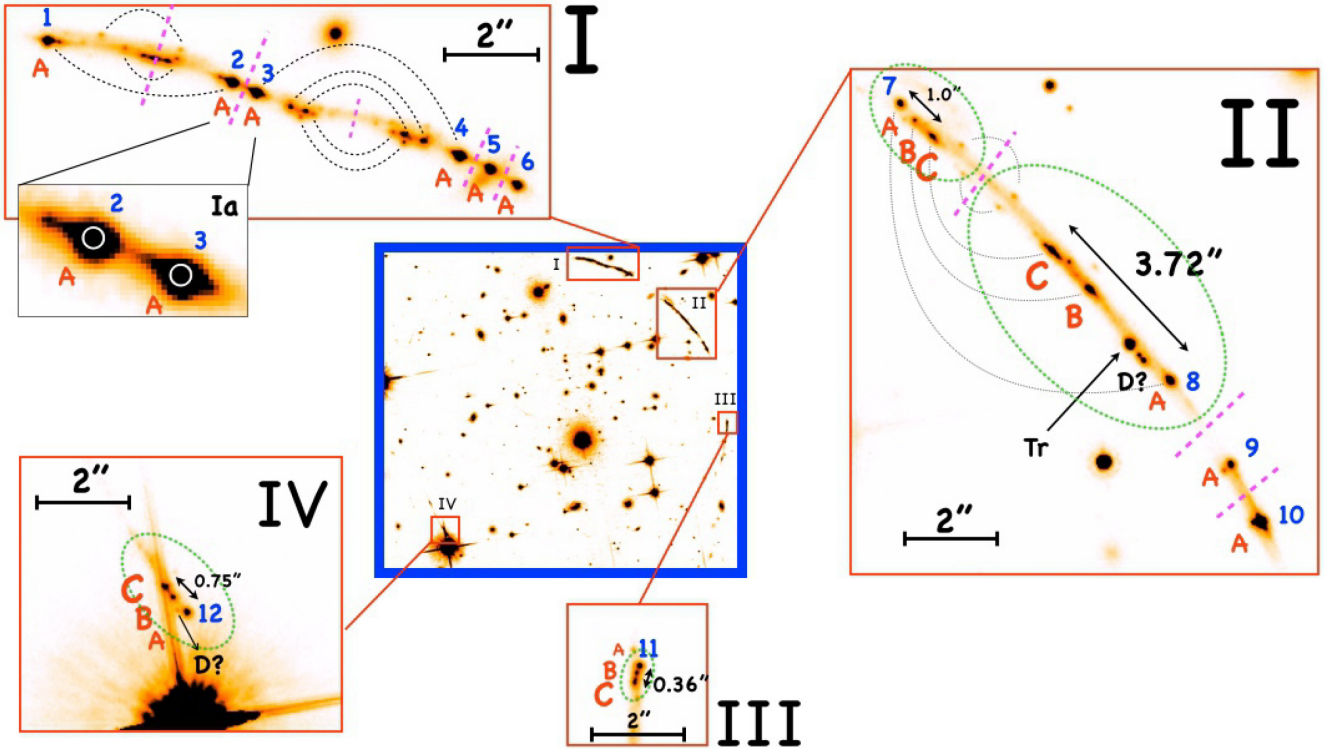
Figure A1. A complete overview of the four arcs is shown in the central panel with the zoomed regions shown clockwise (panels I, II, III, and IV). The tangential stretch is clearly visible after the identification of the three knots A, B, and C. The knot A is the LyC knot discussed in this work and its distinctive signature allows a secure identification (Rivera-Thorsen et al. 2019). In particular, the ratio among the angular separations between A-C for the less magnified system (III) and the most stretched one (II) implies an average tangential magnification larger than 10 for system II (i.e. knowing the arc III has \mu > 1 ). The relative flux ratio among the LyC knots 2 (or 3) and image 8 of \simeq 2 further implies that the magnification for images 2 (or 3) is higher than 20. The magenta dotted lines mark approximately the locations where the critical lines cross the arcs (for the arc I, see also Rivera-Thorsen et al. 2019). The dotted green ellipses highlight the multiple structures containing the knots A, B, and C and other small features. Some of the mirrored multiple images within the arcs (accordingly with the parity of the images generated by strong lensing, Kneib & Natarajan 2011) and tiny SF knots are connected with the dotted black lines. Other substructures are marked with ‘D’ and are visible only in the most magnified regions (or represent foreground sources). Finally, another bright object not present in any of the other arcs is marked as ‘Tr’ in panel II and represents a possible transient (Vanzella et al. in preparation). The inset Ia shows a zoom of the images 2 and 3 and highlights the circular apertures used in Rivera-Thorsen et al. (2019) to derive the F814W magnitudes reported in their table 1. While such a small aperture is appropriate for their goals (measure of the ionizing-to-non-ionizing flux ratio for a point-like object), our magnitudes derived with galfit fitting in the F814W band account for the total flux and spatially resolved morphology, making our estimates closer to the total magnitude.
