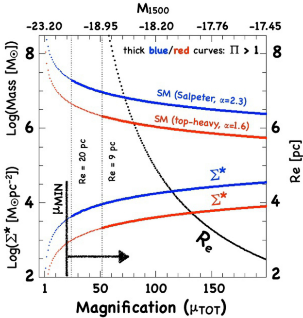
Figure 6. The stellar mass, stellar mass surface density ( \Sigma^* ), and the effective radius ( R_e , on the right Y-axis) of the Sunburst LyC knot are calculated as a function of the total magnification, \mu_{TOT} . The red and blue curves correspond to top-heavy and Salpeter IMF, respectively. The LyC knot becomes compatible with a gravitationally bound star cluster if \mu_{TOT} > 25(50) . This regime ( \Pi > 1 ) is highlighted with the thick lines, where \Sigma^* approaches the values measured in the densest objects known, like globular clusters and young massive clusters. The thick black horizontal arrow in the bottom marks the minimum magnification, \mu_{TOT} > 20 , we estimate in Appendix A.
