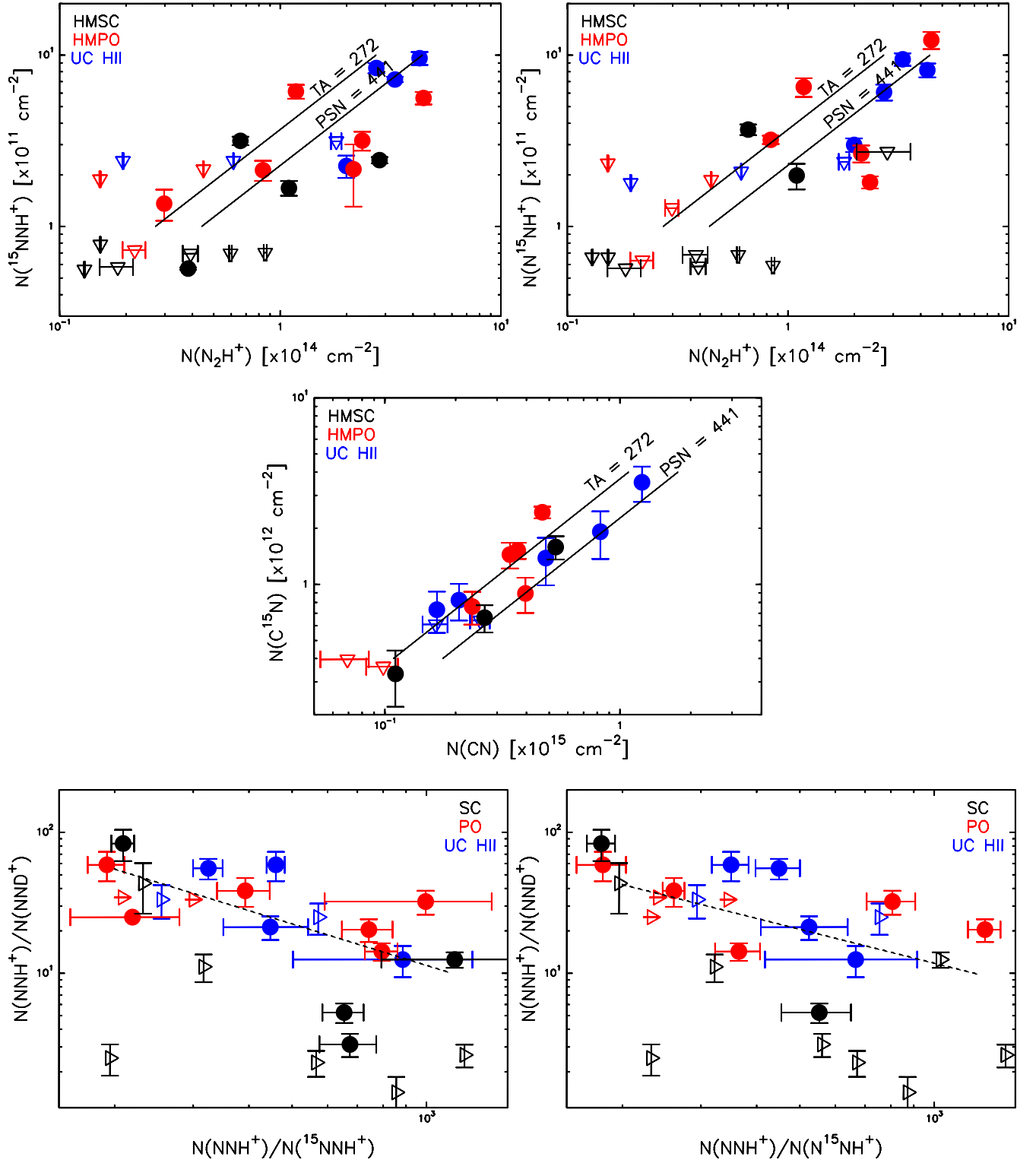
Figure 2. Top panels: column density of \text{N}_2\text{H}^+ against that of ^{15}\text{NNH}^+ (left) and ^{15}\text{NH}^+ (right). Middle panel: column density of CN against that of \text{C}^{15}\text{N} . Bottom panels: comparison between the ^{14}\text{N}/^{15}\text{N} isotopic ratio as derived from the column density ratios N(\text{N}_2\text{H}^+)/N(^{15}\text{NNH}^+) (left) or N(\text{N}_2\text{H}^+)/N(^{15}\text{NH}^+) (right), and the H/D isotopic ratio N(\text{N}_2\text{H}^+)/N(\text{N}_2\text{D}^+) . In all panels, the filled circles represent the detected sources (black = HMSCs; red = HMPOs; blue = UC HII). The open triangles in the top and middle panels correspond to the upper limits on N(^{15}\text{NNH}^+) , N(^{15}\text{NH}^+) , or N(\text{C}^{15}\text{N}) , respectively, while in the bottom panels, they indicate lower limits on either N(\text{N}_2\text{H}^+)/N(^{15}\text{NNH}^+) or N(\text{N}_2\text{H}^+)/N(^{15}\text{NH}^+) . The solid lines indicate the mean atomic composition as measured in the terrestrial atmosphere (TA) and in the proto-solar nebula (PSN; see Hily-Blant et al. 2013a and references therein). The dashed lines in the bottom panels indicate least square fits.
