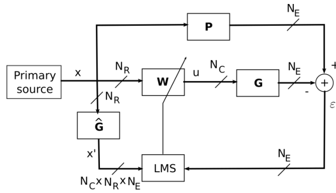
Figure 3 – Fx-LMS scheme. P and G denote the primary and secondary paths; \hat{G} is an estimation of G ; W indicates the set of adaptive filters whose updating is ruled by the LMS algorithm.
