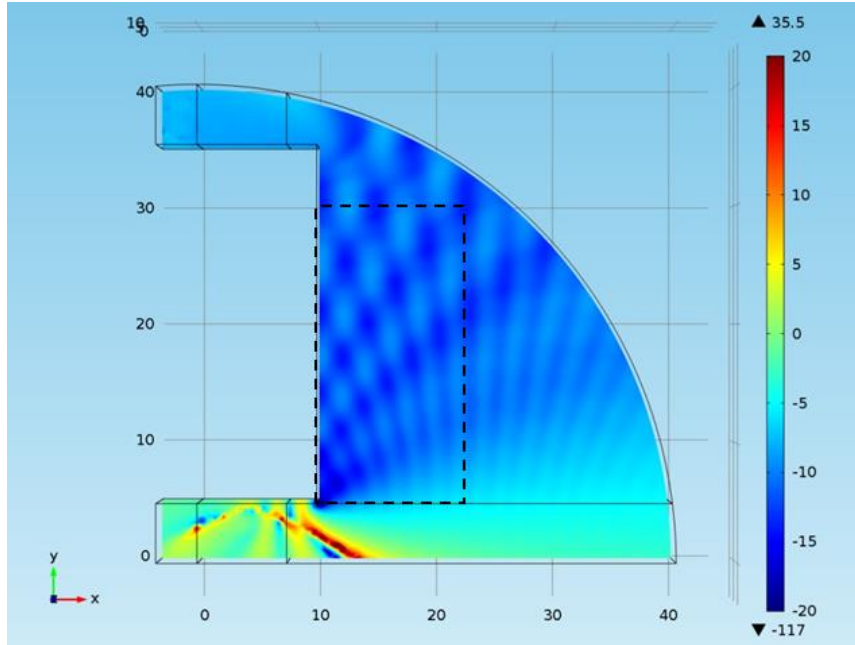
Figure 11 – Noise gain (in dB) after the activation of the ANC system (at 1.7 m from the ground): numerical simulation of a scenario similar to the first experimental tests setting.
