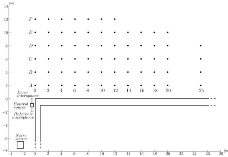
Figure 9 – Top view of the first experimental setting. The noise source is placed on one side of the corner and the error microphones in proximity of the corner edge. The dots indicate the measurement points.
