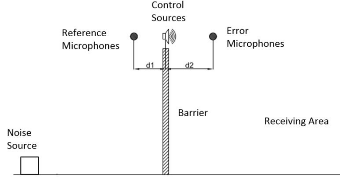
Figure 2 - Testbed layout.
