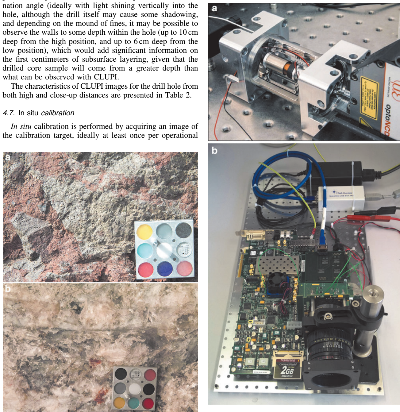
FIG. 16. CLUPI focus mechanism breadboard developed and assembled at the Space Exploration Institute (a) and focal plane assembly breadboard (b) developed by RUAG Space.
