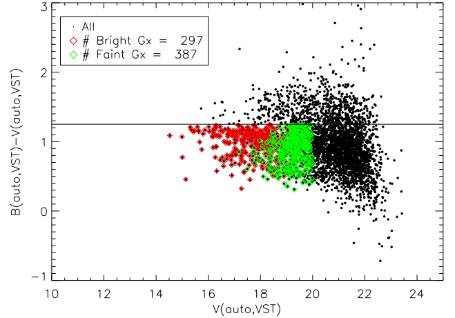
Fig. 1. Candidates for spectroscopic follow-up in A2382: the color cut is set at (B - V) = 1.25 . Black dots are sources flagged as galaxies and red and green symbols indicate galaxies belonging to the bright and faint configurations, respectively.
