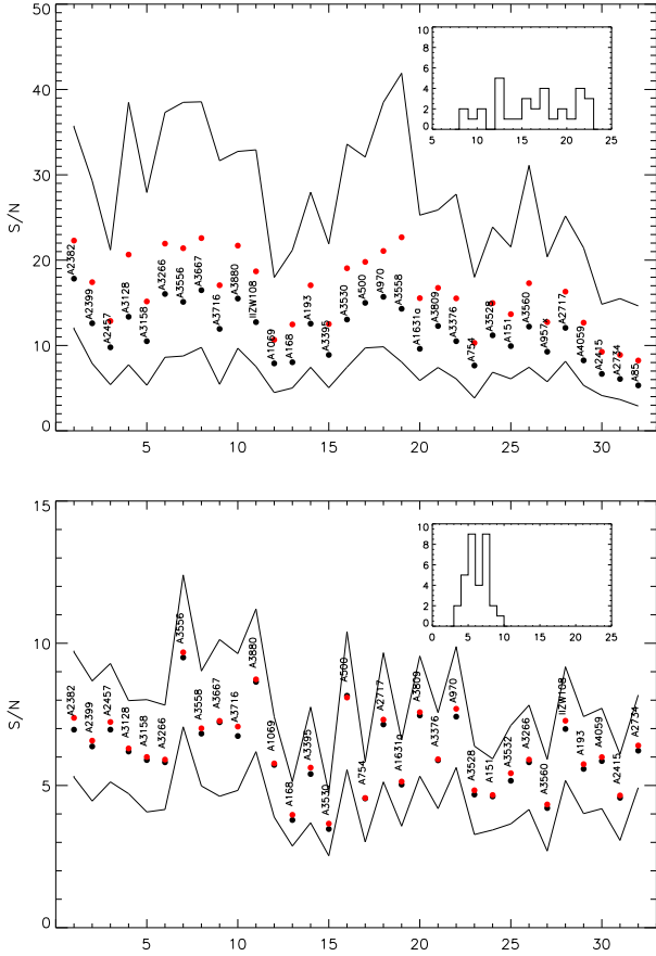
Fig. 2. Mean (red) and median (black) signal-to-noise together with the 68% confidence limits for the bright (top panel) and faint (bottom panel) configurations. In the insets , the average distributions of the measured signal-to-noise in the observed configurations (32 are bright and 32 are faint) are shown.
