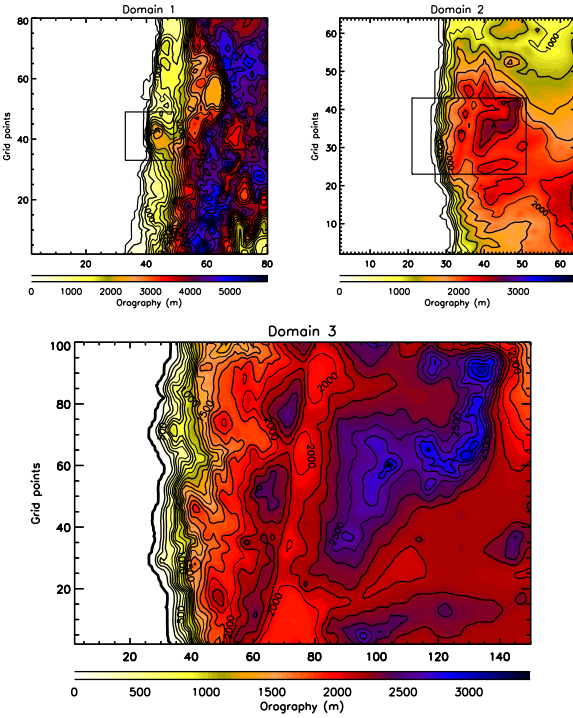
Figure 1. Orography (altitude in m) of the region of interest as seen by the MESO-NH model for all the embedded domains of the model grid-nested configuration. (a) Domain 1 (digital elevation model, i.e. orography data from GTOPO), (b) Domain 2 (digital elevation model from GTOPO), (c) Domain 3 (digital elevation model from ISTAR). ‘P’ stands for Cerro Paranal, ‘A’ stands for Cerro Armazones. The black square in Domain 1 represents the surface of Domain 2. The black rectangle in Domain 2 represents the surface of Domain 3. See Table 1 for the specifications of the domains (number of grid points, domain extension, horizontal resolution).
