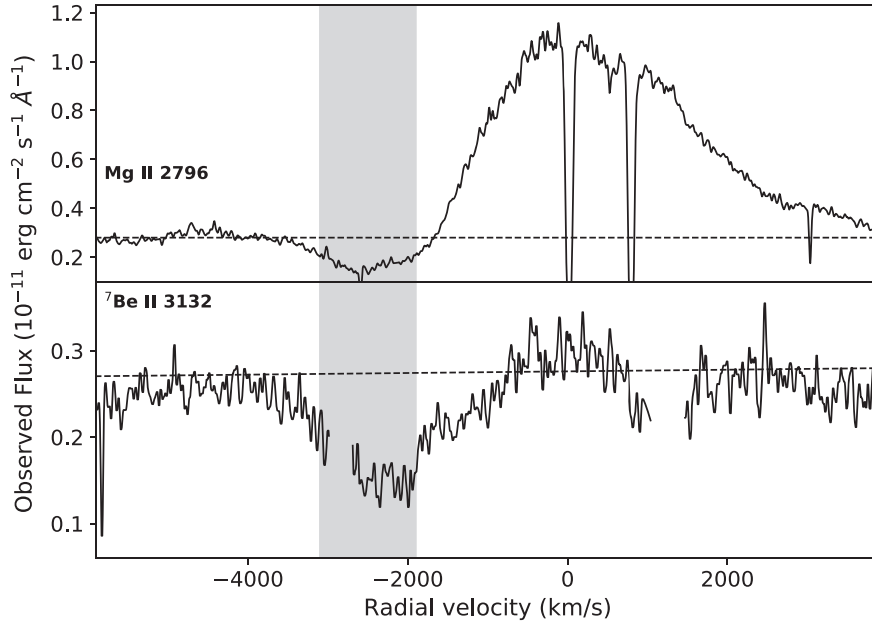
Figure 4. The P Cygni absorptions of the Mg II \lambda 2800 and {}^7\text{Be} II \lambda 3132 lines in the IUE high-resolution spectrum of day 3. Note the similar velocity structure of the two resonant transitions. The gap close to -3000 \text{ km s}^{-1} in the spectrum of {}^7\text{Be} II corresponds to the absence of overlap between two adjacent echelle orders.
