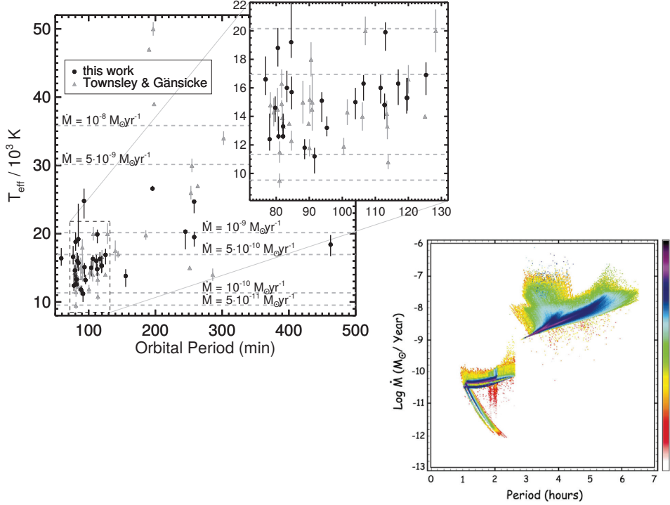
Figure 2. Top : effective temperature as function of the orbital period from this work (black) and from Townesley & Gänsicke (2009, grey). Bottom : present day CV population from Howell et al. (2001). The colour scale gives the logarithm of the system number density. (See online version for a colour figure).
