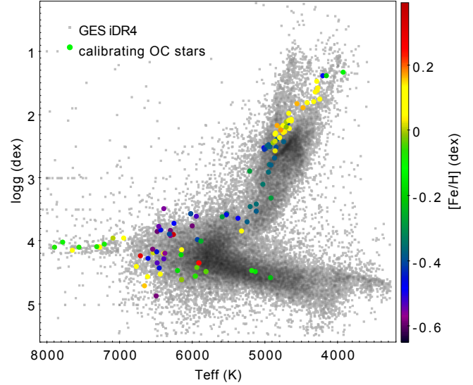
Fig. 13. Position on the T_{\text{eff}} - \log g plane of the stars in calibrating OCs including archival data analyzed in iDR4 (namely NGC 2243, NGC 6705, and NGC 3532) and colored according to their [\text{Fe}/\text{H}] . These stars were observed with the MW field and the OC setups. Of course, many more OC stars are observed with the OC setups alone (on the order of 20 000, see Table 1). The whole GES iDR4 sample is reported in the background as smaller grey dots.
