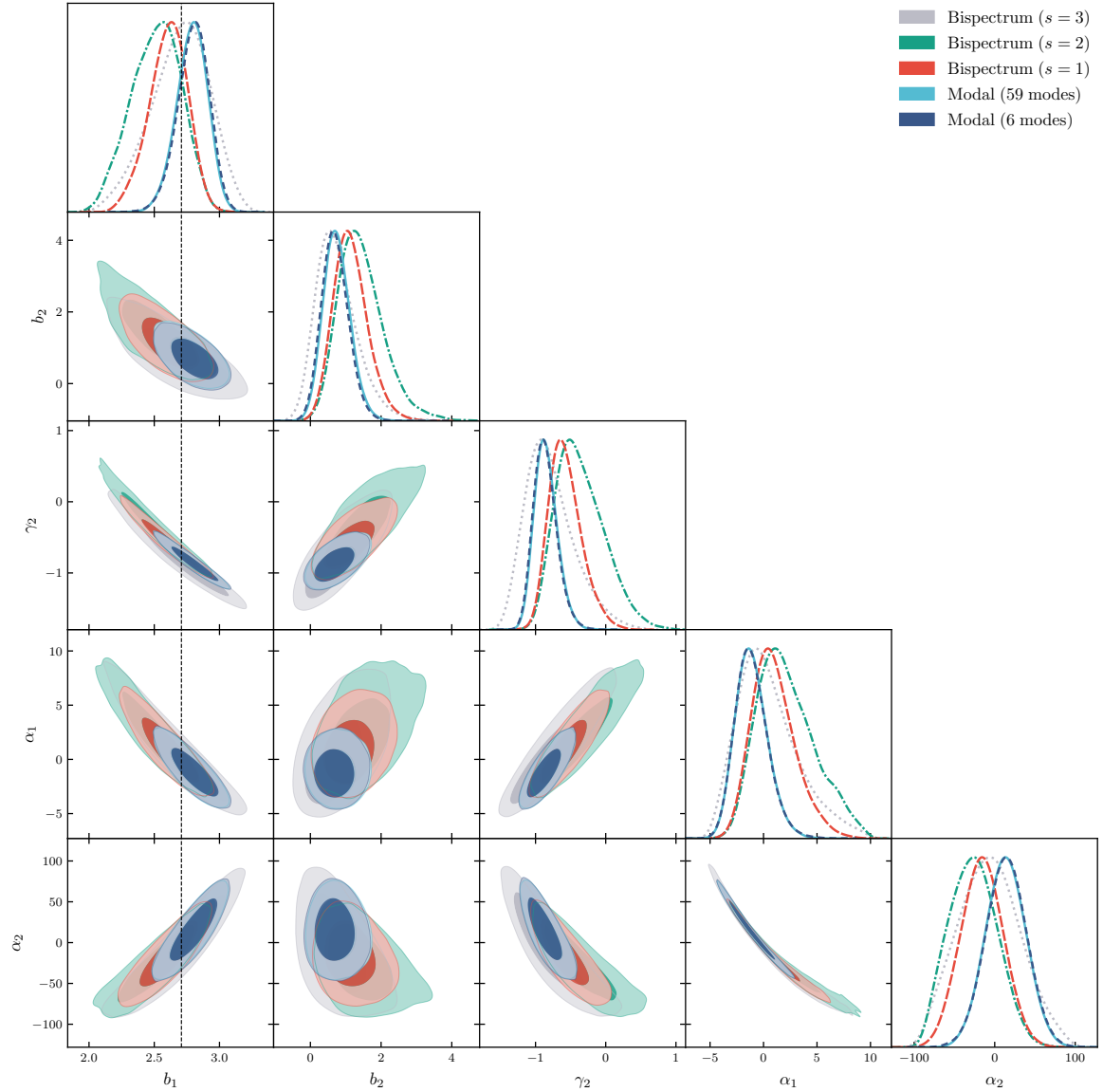
Figure 8: Benchmark comparison between modal bispectrum and standard bispectrum constraints for k_{\text{max}} = 13.5 k_f \approx 0.06 h \text{ Mpc}^{-1} . The vertical dashed black line represents the constraint on b_1 from the large-scale ratio of cross-power spectra P_{hm}/P_{mm} . Standard bispectrum constraints with three different bin sizes are shown: s = 1 (red), 2 (green), and 3 (gray). The modal bispectrum constraints with six modes (dark blue) and 59 modes (light blue) are identical, indicating that the modal bispectrum constraints have already converged with six modes.
