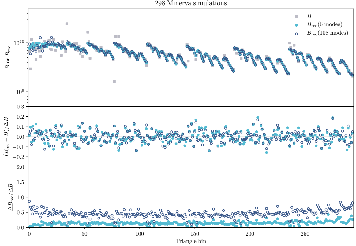
Figure 6: Comparison of the standard bispectrum vs reconstructed bispectrum means and errors over all 298 Minerva simulations for k_{\text{max}} = 13.5 k_f . While the means agree to within \sim 10\% of the error of the standard bispectrum estimator (middle panel), the error in the reconstructed bispectrum is generally suppressed relative to the error in the standard bispectrum measurement (bottom panel). This suppression is larger when fewer modes are used in the reconstruction.
