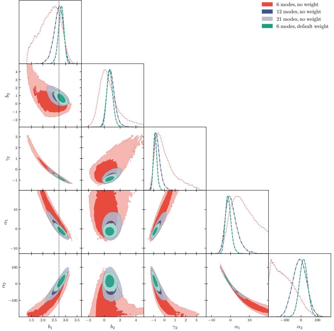
Figure 15: Comparison of modal bispectrum constraints at k_{\text{max}} = 13.5 k_f \approx 0.06 h \text{ Mpc}^{-1} using the benchmark weighting function in eq. (2.6) (green) vs no weight, where w = 1 . When the six custom modes are used in both cases, w = 1 (red) leads to weaker parameter constraints, but this sub-optimal choice of weighting can be fully compensated for by using more modes. For this k_{\text{max}} , 12 modes (dark blue) is not sufficient, but 21 modes (gray, overlapping exactly with the green contours) are able to recover the same constraints as the more optimal weighting.
