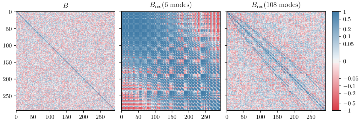
Figure 7: Comparison of correlation matrices from the standard bispectrum and reconstructed bispectra for 294 triangle bins and k_{\text{max}} = 13.5 k_f . The noticeable differences in the correlation matrices for B and B_{\text{rec}} indicate that the covariance matrix for the standard bispectrum estimator cannot be recovered by the modal bispectrum. This discrepancy is especially pronounced when fewer modes are used in the reconstruction.
