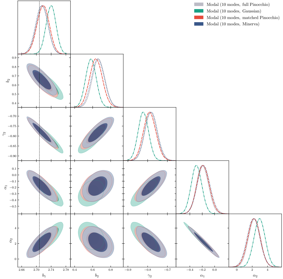
Figure 18: Comparison of parameter constraints when different covariance matrices are used to obtain constraints at k_{\text{max}} = 24.5 k_f \approx 0.10 h \text{ Mpc}^{-1} using 10 modes. The Gaussian covariance matrix (green) leads to biased and underestimated parameter constraints, but the covariance matrices estimated from 298 Minerva simulations (dark blue) and 298 Pinocchio simulations with matched initial conditions (red) are in good agreement with the benchmark modal constraints that used the full set of 10,000 Pinocchio simulations (gray, nearly identical to the dark blue and red contours).
