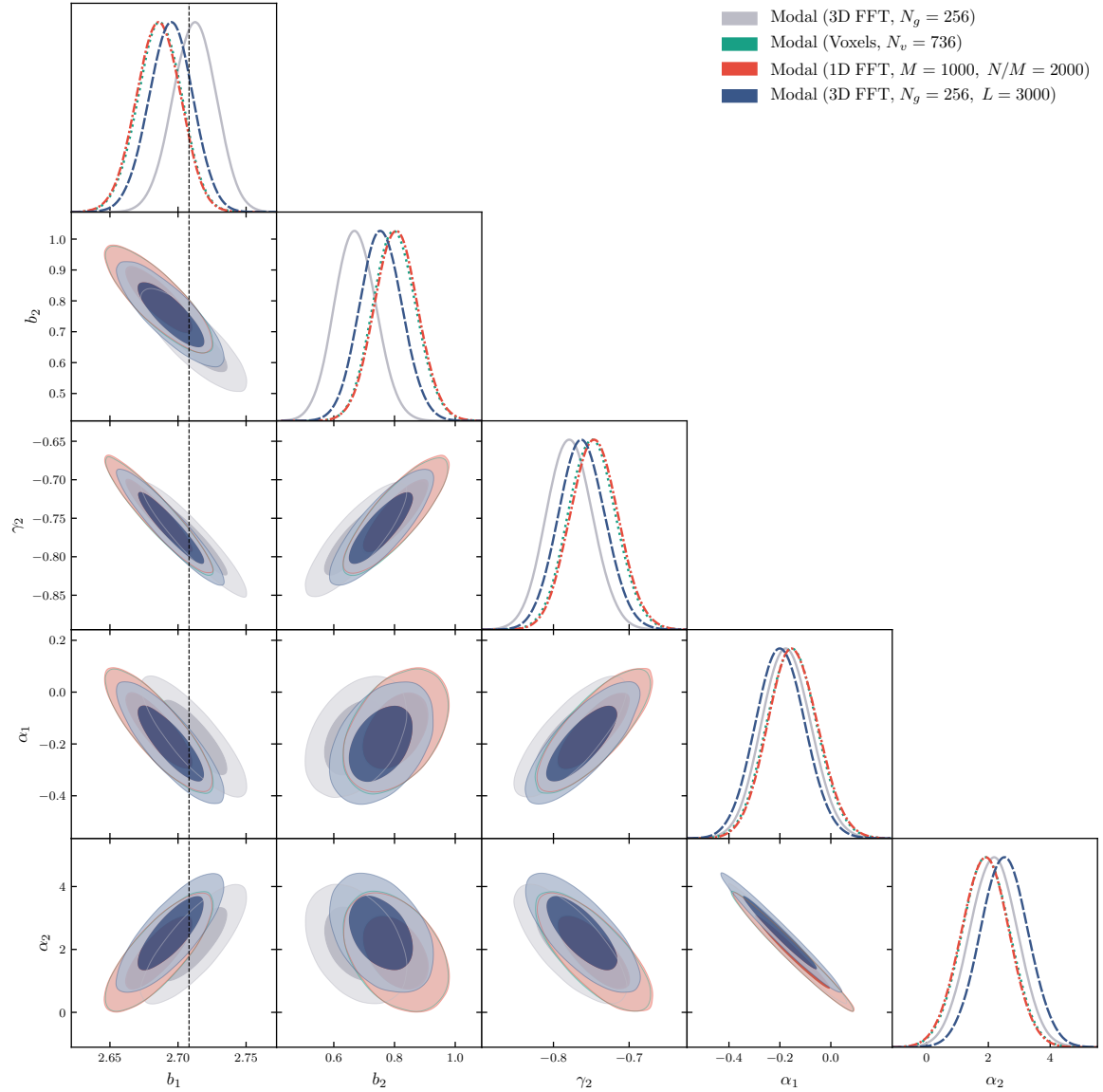
Figure 13: Comparison of modal bispectrum constraints at k_{\text{max}} = 24.5 k_f \approx 0.10 h \text{ Mpc}^{-1} using different inner product methods. As in Fig. 12, the voxel (green) and 1D FFT (red) methods have converged towards each other, and both are biased relative to the correct 3D FFT result (gray). The 3D FFT case with L = 3000 h^{-1} \text{ Mpc} (dark blue) is also biased, illustrating that getting the discretization as in the measurements is important.
