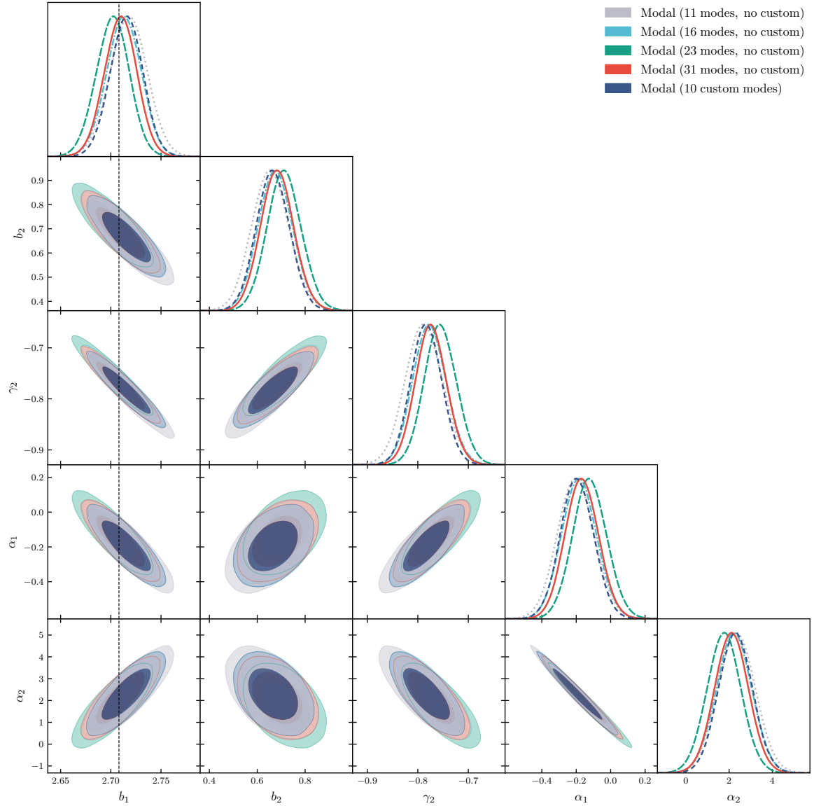
Figure 11: Comparison of modal bispectrum constraints at k_{\text{max}} = 24.5 k_f \approx 0.10 h \text{ Mpc}^{-1} without and with custom modes. We compare constraints without custom modes using 11 modes (gray), 16 modes (light blue), 23 modes (green), and 31 modes (red) with the converged benchmark constraints that used 10 custom modes (dark blue).
