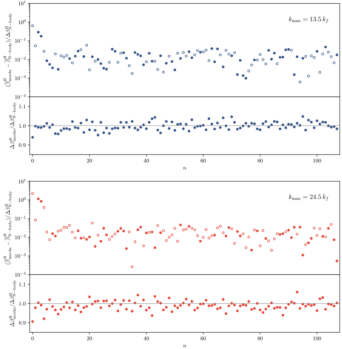
Figure 3: Means and errors of modal expansion coefficients measured from 298 realizations of Pinocchio mock halo catalogs are compared with the same measurements from the Minerva N -body simulations with matching initial conditions. The two panels show the measurements for k_{\max} = 13.5 k_f (top, blue circles) and 24.5 k_f (bottom, red circles). Filled (empty) circles correspond to positive (negative) values. The bottom subplots show that the errors from the mocks are always within 10% of the N -body simulations.
