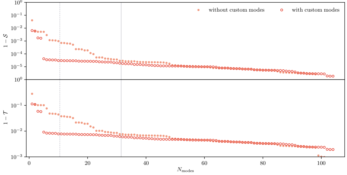
Figure 16: Shape correlator \mathcal{S} (top) and total correlator \mathcal{T} (bottom) for k_{\max} = 24.5 k_f . Smaller values of 1 - \mathcal{S} and 1 - \mathcal{T} correspond to smaller differences in the reconstructed bispectrum compared to the case where the maximum number of modes are used. The vertical gray lines mark N_{\text{modes}} = 10 and 31 , which we previously found was sufficient to obtain robust parameter constraints when custom modes are included or excluded, respectively.
