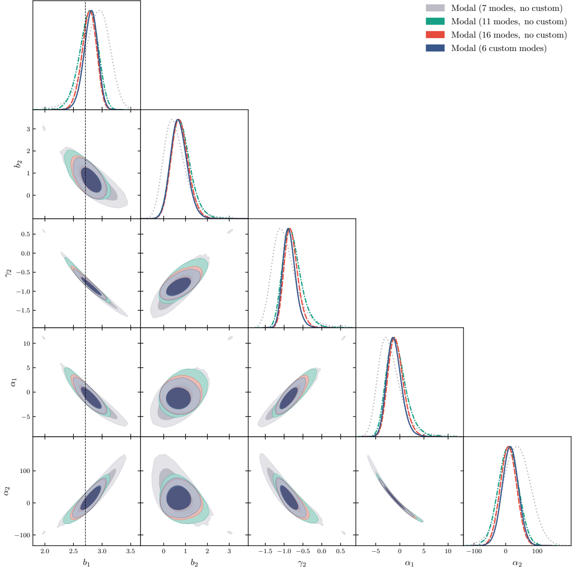
Figure 10: Comparison of modal bispectrum constraints at k_{\text{max}} = 13.5 k_f \approx 0.06 h \text{ Mpc}^{-1} without and with custom modes. We compare constraints without custom modes using 7 modes (gray), 11 modes (green), and 16 modes (red) with the converged benchmark constraints that used 6 custom modes (dark blue).
