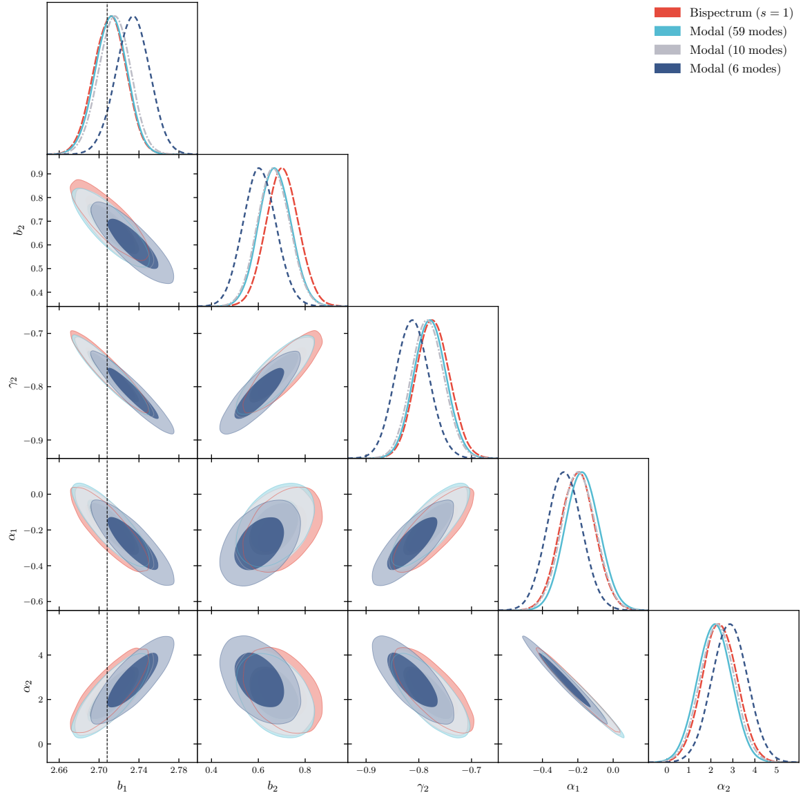
Figure 9: Comparison of modal bispectrum and standard bispectrum constraints at k_{\text{max}} = 24.5 k_f \approx 0.10 h \text{ Mpc}^{-1} . At this k_{\text{max}} , we can only compare with the s = 1 binning of the standard bispectrum estimator (red). By comparing the constraints using six custom modes (dark blue), 10 modes (gray), and 59 modes (light blue), we find that 10 modes are sufficient for the modal constraints to converge, as there is no further change when 59 modes are used.
