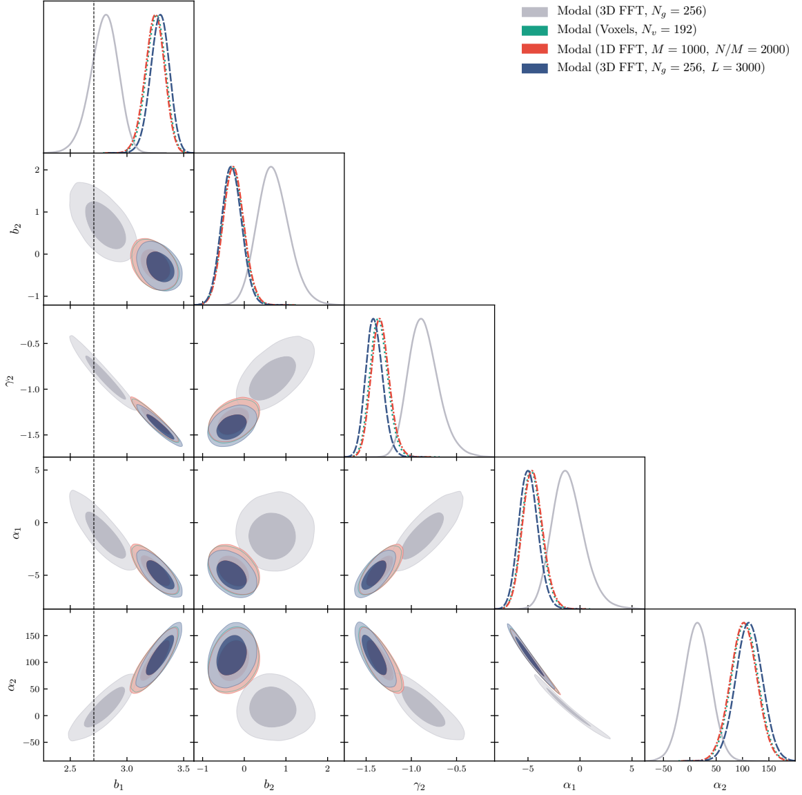
Figure 12: Comparison of modal bispectrum constraints at k_{\text{max}} = 13.5 k_f \approx 0.06 h \text{ Mpc}^{-1} using different inner product methods. The voxel (green) and 1D FFT (red) methods have converged towards each other, and both disagree with the 3D FFT result (gray) that agreed with the standard bispectrum constraint in Fig. 8. The 3D FFT case with L = 3000 h^{-1} \text{ Mpc} (dark blue) is also biased, illustrating that getting the discretization as in the measurements is important.
