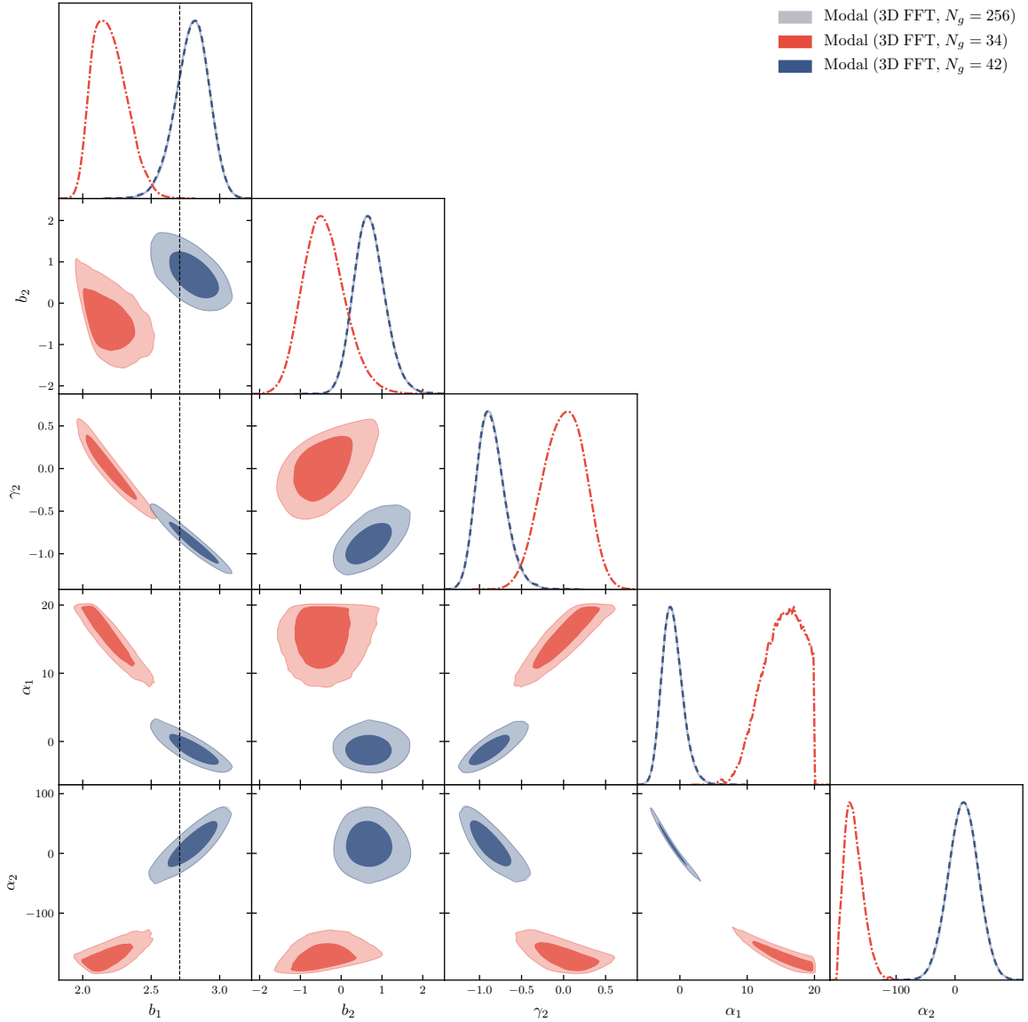
Figure 14: Comparison of modal bispectrum constraints at k_{\text{max}} = 13.5 k_f \approx 0.06 h \text{ Mpc}^{-1} using different FFT grid resolutions, N_g . The case with N_g = 42 (dark blue) yields identical results to the benchmark case with N_g = 256 (gray, hidden underneath the dark blue contours), because both satisfy N_g > 3k_{\text{max}}/k_f \approx 41 , while N_g = 34 (red) is insufficient and leads to incorrect constraints.
