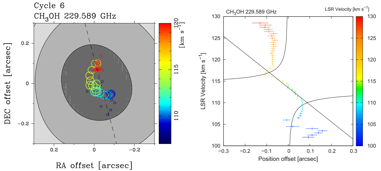
Fig. 10. (Left) Velocity-centroid map of the CH 3 OH 229.589 GHz (15 4 –16 3 E) lines in Cycle 6. The contours and gray-scale image show the moment 0 map. Peak intensities and positions are measured using the channel map produced with the whole UV range and the finer spectral resolution of 0.5 km s −1 . The size of each circle is proportional to the intensity. The dashed line indicates the position angle of the linear distribution of the centroid positions (15°). The (0, 0) position corresponds to RA = 18 h 35 m 08 s .140 and Dec = −07°35′04″.15 (J2000.0). (Right) Position–velocity (PV) diagram of the CH 3 OH 229.589 GHz (15 4 –16 3 E) line for the Cycle 6 data produced from the velocity centroid map. The position offset is measured along the dashed line indicated in the velocity-centroid map (left-hand panel). A solid line shows the best-fitting linear velocity gradient between 110 and 117 km s −1 , with the enclosed mass of 8.8 M ⊙ .
