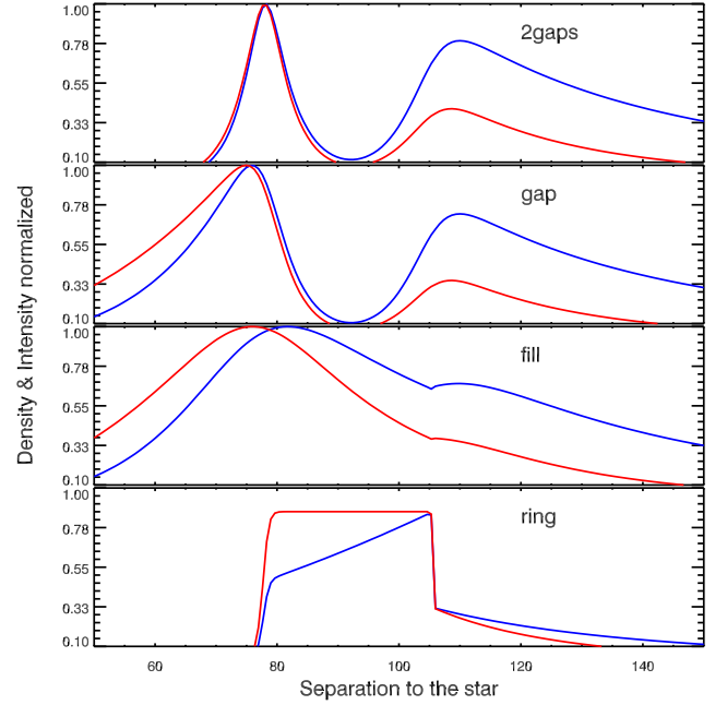
Fig. 5. Examples of the density (blue) and intensity (red) functions corresponding to the four model families.
