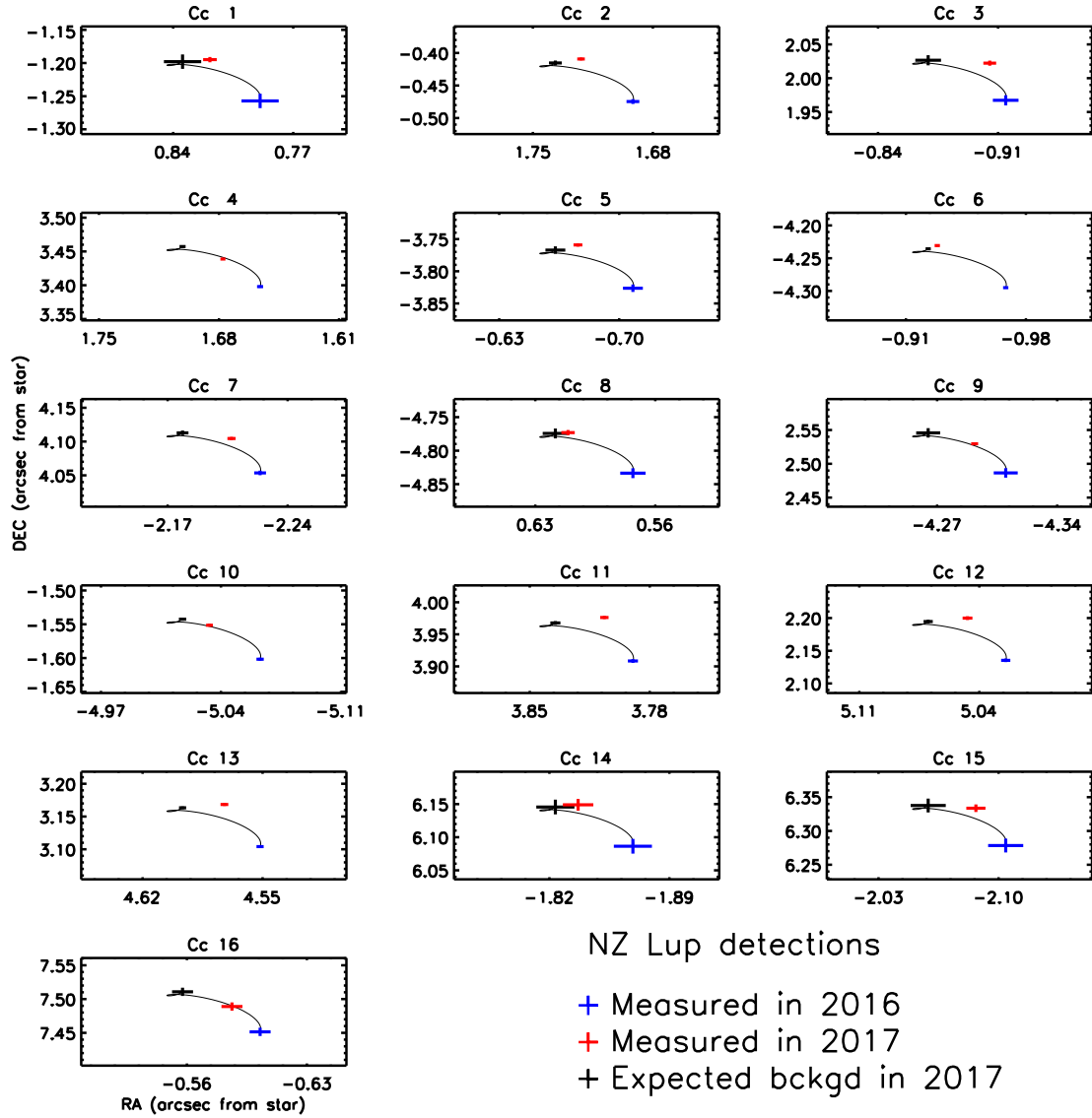
Fig. E.2. Positions of all points sources in the IRDIS field of view as measured at two epochs (2016-05-31 and 2017-04-30) compared to the expected positions if they were background stars.
