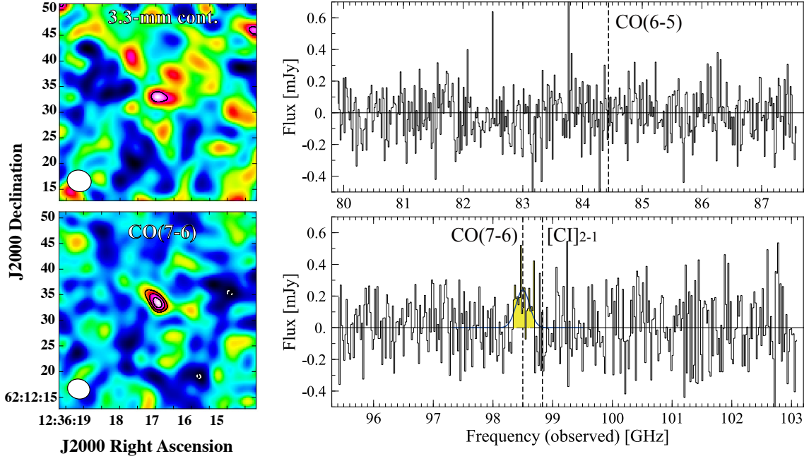
Extended Data Figure 4 | NOEMA 3-mm observation results. Left, 3.3-mm continuum (top) and the velocity-integrated CO(7-6) maps with the natural weighting. The black (white) contours are drawn at 3\sigma , 4\sigma , and 5\sigma ( -3\sigma ). Right, NOEMA 3-mm band spectrum for LSB (top) and USB (bottom) with a 2.''0 radius aperture. The dashed vertical line indicates the observed frequency of the expected far-IR lines based on the source redshift of z = 7.1899 determined by the [C II] line. The blue curve is the best-fit Gaussian for the CO(7-6) line. The yellow shade indicates the velocity range used for the velocity-integrated map in the left panel.
