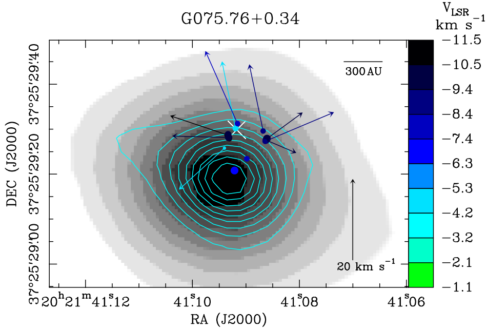
Fig. 6. Gray-scale image: JVL A-Array C-band continuum, using gray-tone steps that increase linearly with the map intensity from 0.037 to 0.37 mJy beam -1 . The JVL A-Array Ku-band continuum is represented with cyan contours with plotted levels -10% and from 10% to 90%, in steps of 10%, of the peak value of 0.50 mJy beam -1 . This source was not observed in the K-band by the JVL A. Colored dots and arrows have the same meaning as in Fig. 1. The amplitude scale for the maser velocity is indicated by the black arrow in the bottom right of the panel. The white cross gives the (velocity-averaged) position of the 6.7 GHz methanol masers, detected at low velocity resolution in C-band.
