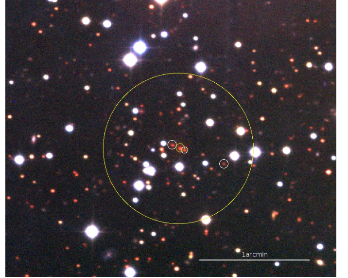
Fig. 9. RGB image of PSZ1 G138.60-10.85, obtained with the WFC/INT. The small white circles show the location of our four spectroscopically confirmed galaxies at z = 0.702 with OSIRIS/GTC. The yellow circle indicates the location of the cluster, and its diameter corresponds to 0.5 Mpc at that redshift.
