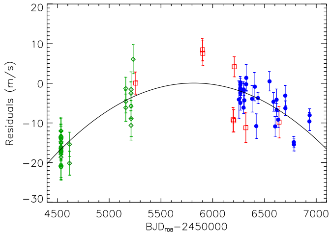
Fig. 11. Long-term trend found in the RV residuals data of XO-2N b after removing the orbital signal of XO-2N b, caused either by a long-period companion XO-2N c or by the activity cycle of the star. Green diamonds, red squares, and blue circles indicate the HDS, HIRES, and HARPS-N measurements, respectively, while the black solid line shows the best fit of the quadratic trend. Residuals of RV measurements with an error bar greater than 5 \text{ m s}^{-1} , even though considered in the analysis, were not included in this plot for a better visual representation of the long-term trend.
