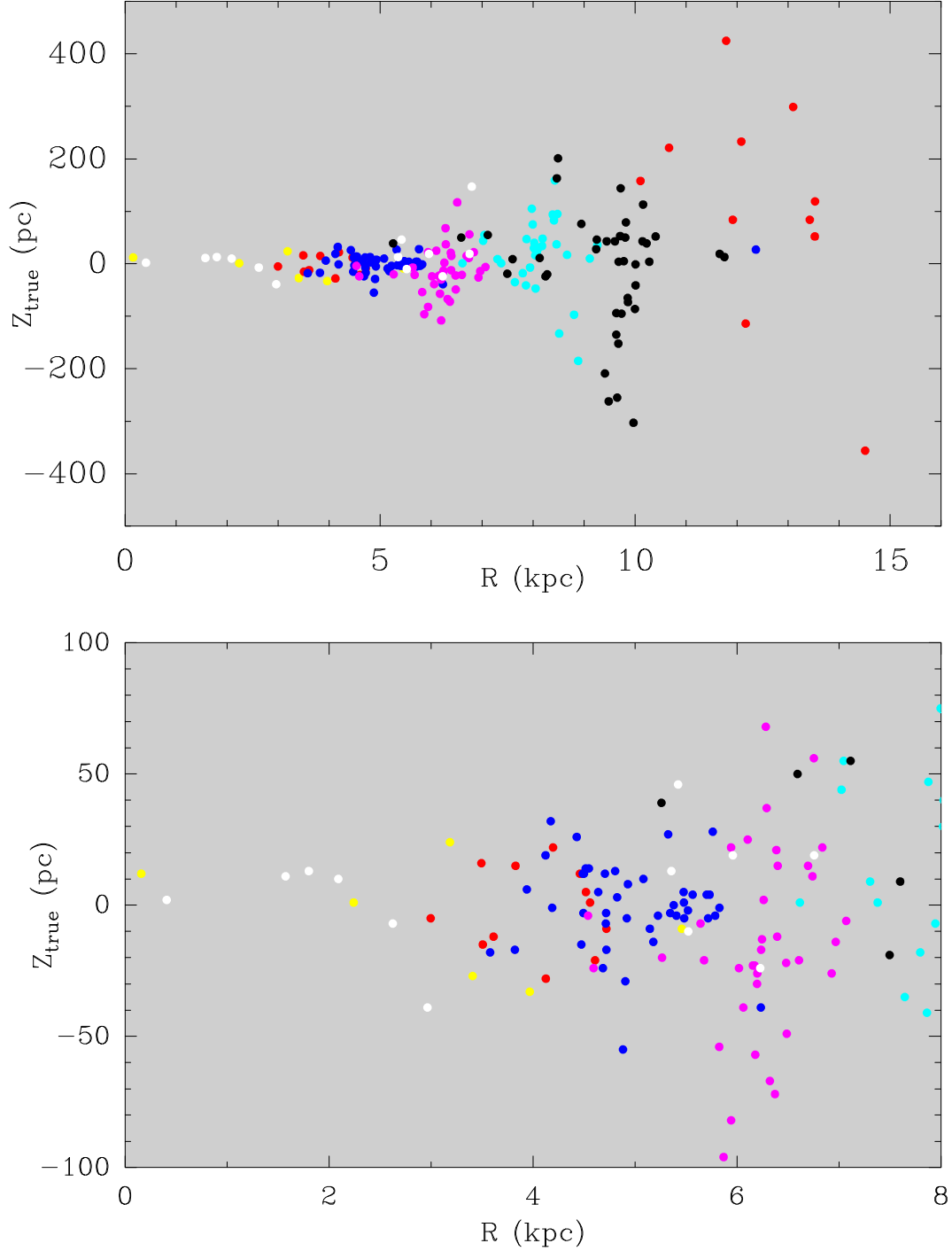
Fig. 5.— The true Z -distribution of young high-mass stars perpendicular to the Galactic plane as a function of Galactocentric radius. Sources are color-coded by spiral arm as in Fig. 1, and Z_{\text{true}} values are corrected for our view from 5.5 pc above the plane, assuming the orientation of the IAU plane. Top panel: All stars in Table 1 with Galactocentric radii less than 16 kpc. Bottom panel: A zoomed view of sources within R = 8 kpc and |Z| < 100 pc.
