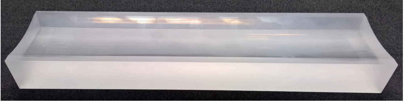
Fig. 9: one of the two paraboloidal mirrors procured from Carl Zeiss SMT GmbH, after the preliminary grinding. The mirror was subsequently lapped to smooth the periodic pattern left after grinding.
