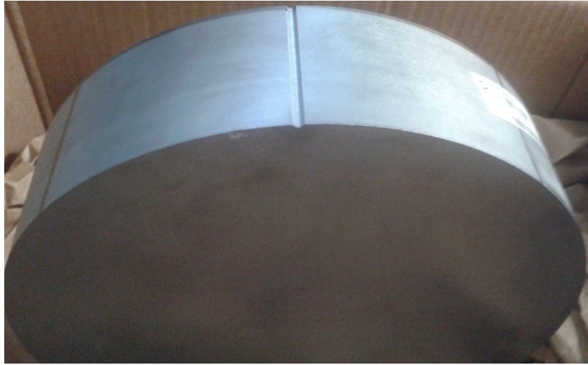
Fig. 11: the monocrystalline cylinder in silicon purchased from MEMC (20 cm diameter, 50 mm thick). The terminal surfaces are the planes (100). The lateral groove locates the (010) planes.
