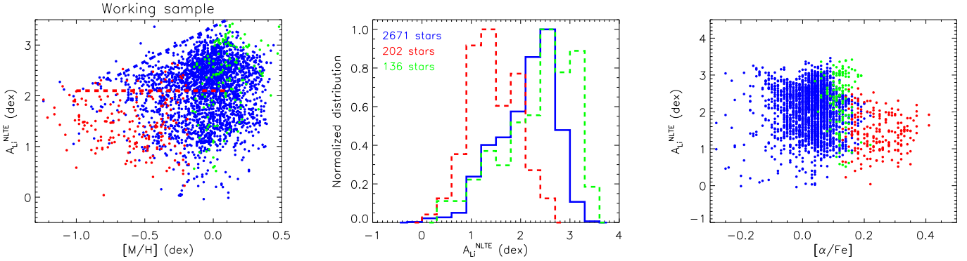
Fig. 11. A_{\text{Li}}^{\text{NLTE}} as a function of [M/H] (left) and its normalized distribution (centre) of the AMBRE/LI stars for the working sample . The thin disc stars are plotted in blue, thick disc members in red and metal-rich \alpha -rich stars in green. The upper envelope of both discs from Ramírez et al. (2012) are shown as dashed lines (bottom, left). We also show A_{\text{Li}}^{\text{NLTE}} vs. [\alpha/\text{Fe}] in the right panel (Spearman’s rank correlation coefficient equal to -0.03 and -0.04 for the thin and the thick disc, respectively).
