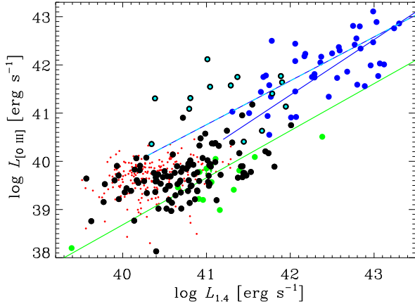
Fig. 4. Radio (NVSS) vs. [O III] line luminosity of the FRIICAT (black), FRIICAT (red), 3C-FR I (green), and 3C-FR II samples (blue). The green line (blue) shows the linear correlation between these two quantities derived from the FR Is (FR IIs) of the 3C sample from (Buttiglione et al. 2010). The dashed blue-cyan line is instead the linear fit on both the 3C and the FRIICAT HEGs.
