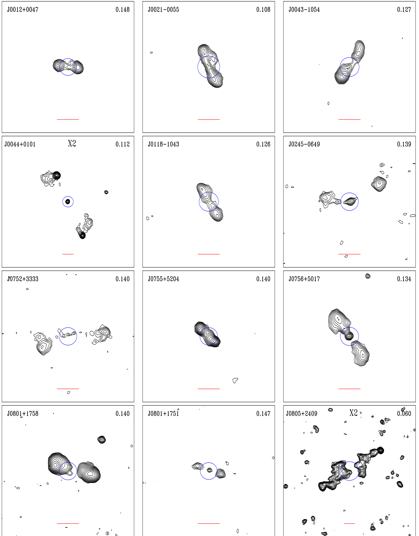
Fig. A.1. Images of the FR IIs selected. Contours are drawn starting from 0.45 mJy/beam and increase with a geometric progression with a common ratio of \sqrt{2} . The field of view is 3' \times 3' in most cases, except for those marked with a 'X2' at the top; the red tick at the bottom is 30'' long. The blue circle is centered on the host galaxy and has a radius of 30 kpc. The source ID and redshift are reported in the upper corners.
