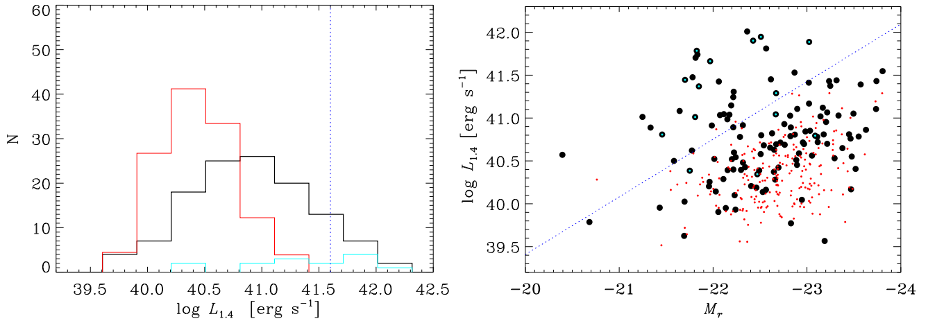
Fig. 3. Left panel: radio luminosity distribution of the FRIICAT (black, cyan for the HEGs) and FRICAT sources (red). The dotted vertical line indicates the transition power between FR I and FR II reported by Fanaroff & Riley (1974). Right panel: radio luminosity (NVSS) vs. host absolute magnitude, M_r , for FRIICAT and FRICAT (black and red, respectively; cyan for the HEG FR II). The dotted line shows the separation between FR I and FR II reported by Ledlow & Owen (1996) to which we applied a correction of 0.34 mag to account for the different magnitude definition and the color transformation between the SDSS and Cousins systems.
