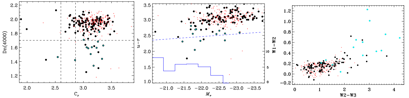
Fig. 2. Left: concentration index C_r vs. Dn(4000) index for the FRIICAT and FRICAT samples indicated by black and red dots, respectively. The HEG FR II are represented by cyan circles. Center: absolute r -band magnitude, M_r , vs. u-r color. Right: WISE mid-IR colors.
