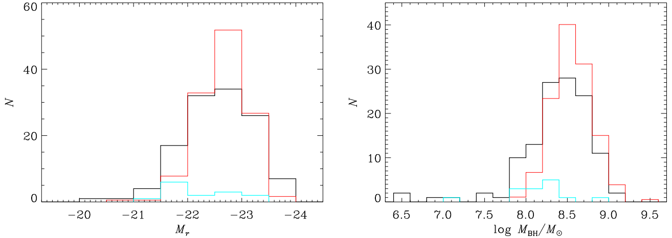
Fig. 1. Distributions of the r -band absolute magnitude ( left ) and black hole masses ( right ). The black histograms are for FRIICAT (cyan for the HEG FRIICAT subsample), the red histograms for the FRICAT. The FRICAT histograms are all scaled by the relative number of FR I and FR II, i.e., by 122/219.
