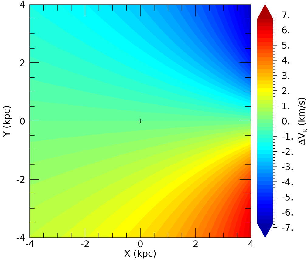
Figure 1. The systematic error in V_R , with respect to heliocentric position (X-axis toward the GC and Y-axis in the direction of Galactic rotation), assuming R_0 = 8.34 kpc in the case that the true R_0 = 8.122 kpc, for a constant circular velocity V_0 = 240 \text{ km s}^{-1} . The systematic error in V_\phi will be of the same magnitude but opposite sign.
