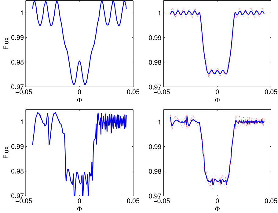
Figure 15. Left panels: simulations of normalized raw light-curves with different systematic effects, due to pointing jitter and strong intra-pixel variations. Jitter time series are: (top) sinusoidal and (bottom) successive smooth sawtooths with increasing frequency. Right panels: Correspondent detrended light curves with (blue) pixel-ICA method and (red, dashed) traditional pixel-phase method. Note that ICA method outperforms the pixel-phase method, with lower residual systematics and retrieved parameters closer to the true values.
