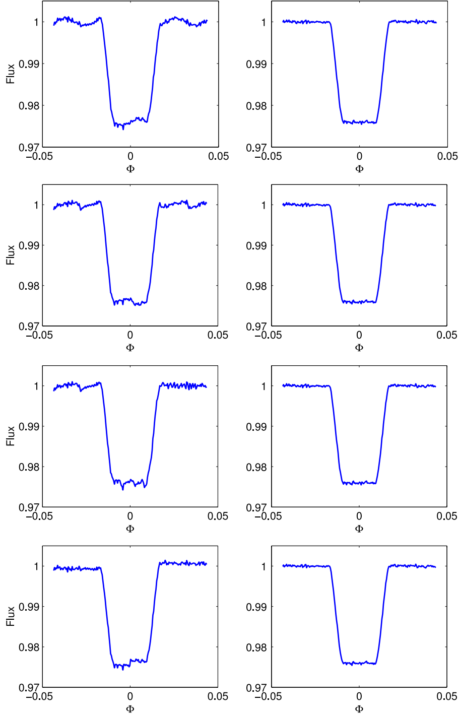
Figure 14. Left panels: simulations of normalized raw light-curves with different systematic effects, due to pointing jitter and different pixel responses. Jitter time series are, from top to bottom: sinusoidal, periodic sawtooth (smoothed), successive smooth sawtooths with increasing frequency, and sudden shift. Right panels: correspondent detrended light curves with pixel-ICA method. Retrieved parameters are consistent with the values adopted to generate the raw light curves.
