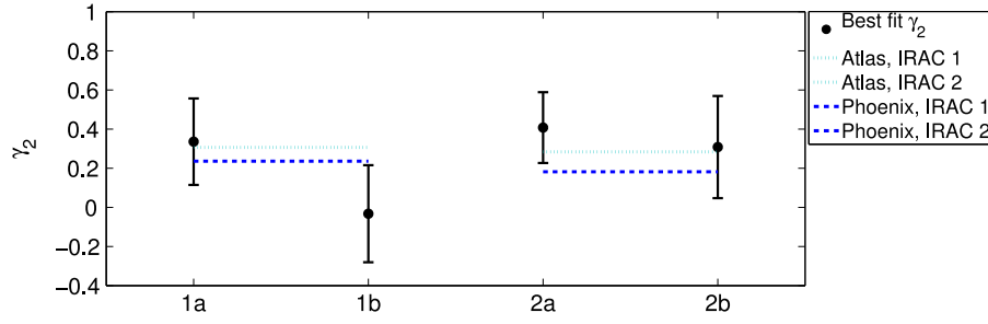
Figure 17. Best fitted values of the quadratic limb darkening coefficient ( \gamma_2 ) for the four observations, assuming \gamma_1 = 0 .
