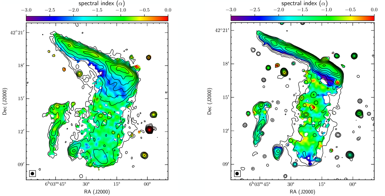
Fig. 11. Spectral index map of the radio halo in 1RXS J0603.3+4214 at 15''/7 resolution. Left: low-frequency (150 and 650 MHz) spectral index map. Contour levels are from the LOFAR and drawn at \sqrt{[1, 2, 4, 8, \dots]} \times 4\sigma_{\text{rms}} . Right: high-frequency (1.5 and 3 GHz) spectral index map. Contours are from the VLA L -band and are drawn as in the left panel . These maps confirm a remarkably uniform spectral index distribution across the halo C between 150 MHz and 3 GHz. It is evident that the relic+halo region shows spectral steeping at low frequencies while there is a uniform spectral index distribution at high frequencies. These maps were created using images IM10, IM13, IM18, and IM21 (see Table 2 for image properties). The color bar shows spectral index \alpha .
