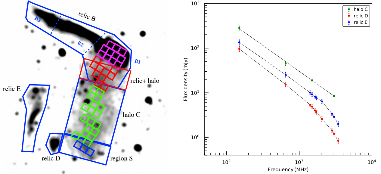
Fig. 6. Left: VLA 15'' resolution image depicting the regions where the integrated flux densities were measured. Right: integrated spectra of the halo C and relics E and D. The spectrum of the halo C is well described by a single power-law spectrum. Relics E and D show spectral steepening beyond 1.5 GHz. The flux densities are measured from 15'' resolution images created using uniform weighting with a uv-cut at 0.4 k\lambda .
