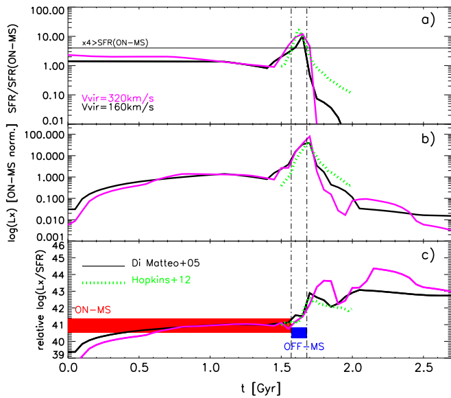
Figure 3. Comparison of our results with predictions of hydrodynamical models that simultaneously follow star formation and the growth of black holes during a galaxy–galaxy merger (di Matteo et al. 2005; Hopkins et al. 2012). (a) To define the simulated merger/starburst phase we report the SFR history of the models normalized to the pre-merger phase. The temporal window where (\text{SFR})/(\text{SFR pre-merger}) is larger than a factor of 4 for all models is marked by the two vertical dot-dashed lines. (b) Evolution of the X-ray luminosity with time. (c) Evolution of the X-ray luminosity to SFR ratio, as a function of time. Two different values of the virial velocity of the collisional galaxies are considered in the di Matteo et al. (2005) model ( v = 160 \text{ km s}^{-1} black lines, v = 320 \text{ km s}^{-1} magenta lines). Our results are presented as a red rectangle for the pre-merger phase (corresponding to our MS normal star-forming sources) and as a blue region for the merger phase (i.e., our starburst sample). The width of L_X/\text{SFR} from our data spans the full range covered in all mass bins (see Figure 1, bottom panel).
