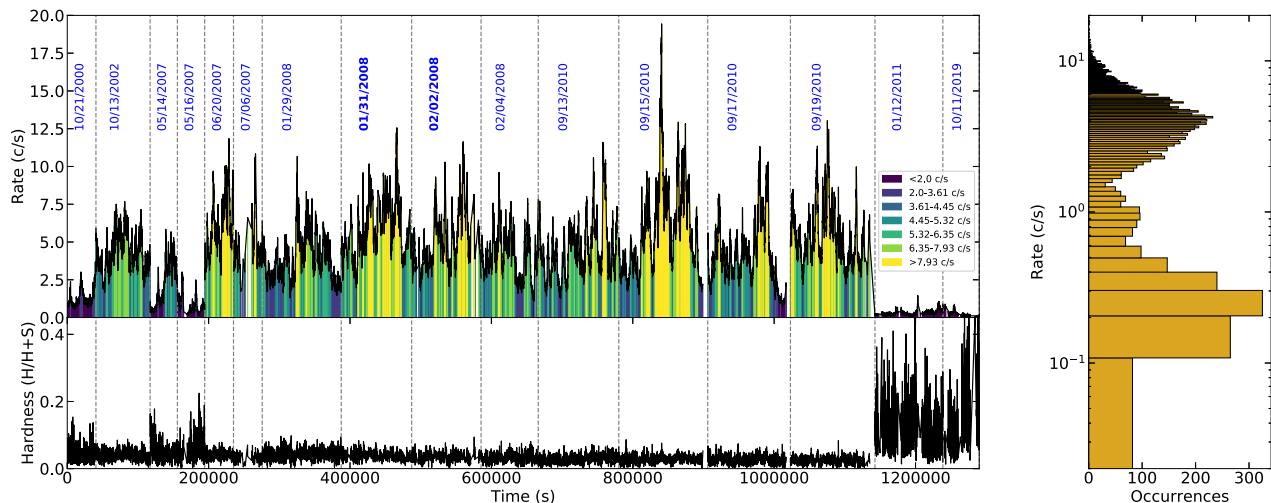
Figure 1. Upper left: An overall EPIC-pn light curve (0.3–10 keV) from 2000 to 2019, where the time gaps between observations are ignored and the observation dates are marked. The vertical dashed lines indicate the begin and end time for each observation. The colours represent the different flux intervals, which have comparable counts. Lower left: The corresponding X-ray HR of the EPIC-pn light curve. S and H denote the counts in the soft and hard energy bands defined as 0.3–2 and 2–10 keV, respectively. Right: The count rate histogram.
