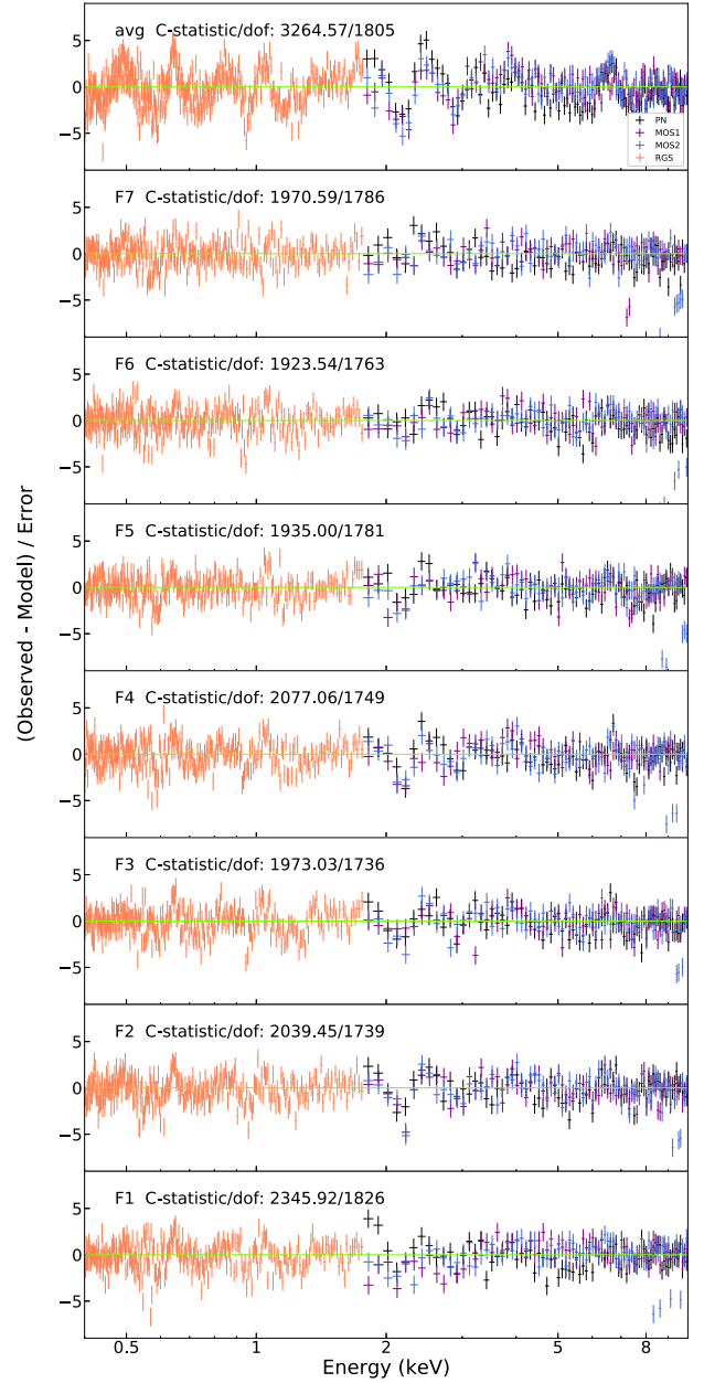
Figure A2. The residuals for the time-average ( top ) and flux-resolved (ordered according to the count rates from bottom to the second panel) spectra with respect to a phenomenological model \text{hot*reds*}(\text{pow}+\text{bb}+\text{laor}*(\text{delt}+\text{delt})) . The Cash statistics and the degree of freedom (dof) are marked as well.
