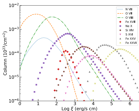
Figure 8. The predicted column densities of different partially ionized ions in a photoionized plasma versus the ionization parameter assuming N_H = 10^{24} \text{ cm}^{-2} and the time average SED (see Fig. 4).
