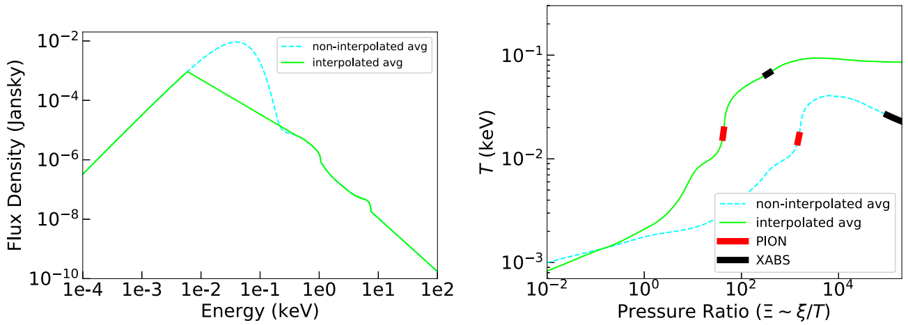
Figure A5. The time-average non-interpolated SED (left) predicted by models and the corresponding stability curve (right) compared with the interpolated SED and its stability curve. The ionization parameters of the photoionized absorber (black) and emitter (red) for each SED are also shown on to the curves.
