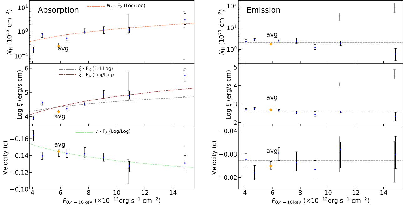
Figure 6. The column density ( Top ), ionization parameters ( Middle ), and velocities ( Bottom ) of the photoionization absorbing ( Left ) and emitting ( Right ) plasmas versus the absorbed X-ray fluxes of the flux-resolved spectra. The uncertainties within the 68 per cent confidence level are shown in black . The time-average results are also marked and shown with orange points. The linear function fits with (1:1 log) and without (log/log) a slope fixed at unity are performed in a logarithmic space for the ionization parameters of the absorbing gas, and also for the logarithmic of the column density and the absolute value of the velocity of the absorber (log/log). The black horizontal dash lines on right-hand panels display the average values of parameters calculated from those of flux-resolved points, indicating a more or less stable emitting gas. Another solution ( grey ), which is comparable in statistics, is also shown in the plots, and its flux is slightly shifted for clarity.
