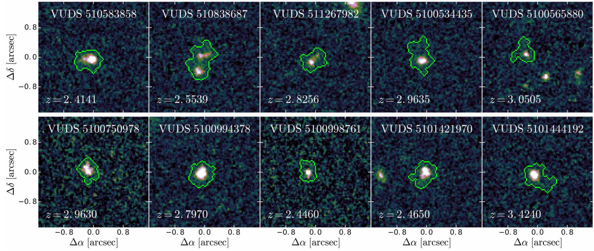
Fig. 2 | The UV morphologies. HST-ACS F814W (FWHM \sim 0.03") postage stamps of the ten galaxies of the sample. At the redshift of the galaxies, F814W corresponds approximately to the rest-frame near-ultraviolet (NUV) band. The green contour show, for each sample galaxy, the isophote containing 100% of the light included in the detection images (Methods). All the galaxies are extremely compact, showing one or two bright star forming clumps in a very low-surface brightness irregular component (limiting AB magnitude of 27.2; Methods). From the top-left to bottom-right corners we identify tadpole shapes (#1, 2, 3, 4, 9, 10), close pairs (#2, 5), and single clumps (#6, 7, 8), which illustrate the morphological diversity of the sample.
