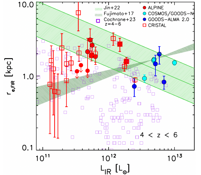
Fig. 4. Effective radius, r_{\text{e,FIR}} vs. IR luminosity, L_{\text{IR}} , at 4 < z < 6 for this sample and from the literature. Red circles represent the results of the ALPINE survey; blue circles the GOODS-ALMA 2.0 survey (Gómez-Guijarro et al. 2022a); cyan circles the super-deblended catalogs in the COSMOS and GOODS-North fields (Jin et al. 2022); and open red squares the CRISTAL survey (Mitsuhashi et al. 2023). The dark green shaded region represents the 1\sigma range of the relation found by Fujimoto et al. (2017). The green lines and the shaded region represent the relation and its 1\sigma dispersion found by Jin et al. (2022). The empty pink squares are simulation results from Cochrane et al. (2023) in the range 4 < z < 6 .
