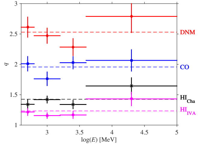
Fig. 6. Spectral variation, relative to the local interstellar spectrum q_{\text{LIS}} , of the \gamma -ray emissivities obtained for the local gas components in the \gamma + A_{VQ} analysis. The q_{\text{CO}} value is given in units of 10^{20} \text{ cm}^{-2} \text{ K}^{-1} \text{ km}^{-1} \text{ s} , q_{\text{DNM}} in 8 \times 10^{20} \text{ cm}^{-2} \text{ mag}^{-1} , and the H I emissivities refer to the optically thin H I case. The dotted lines mark the mean emissivities.
