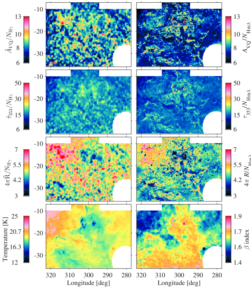
Fig. 11. Three upper rows: spatial variations of the dust properties per gas nucleon with the total gas measured by N_{H\gamma} on a 0.375 pixel grid (left) and by N_{Hm\lambda} on a 0.125 pixel grid (right). Lower row: colour temperature and \beta index of the dust SED, measured at 5' resolution by Planck Collaboration XI (2014) and displayed on a 0.125 pixel grid. The A_{VQ}/N_H values are in units of 10^{-22} mag cm ^2 , \tau_{353}/N_H in 10^{-27} cm ^2 , and 4\pi R/N_H in 10^{-31} W.
