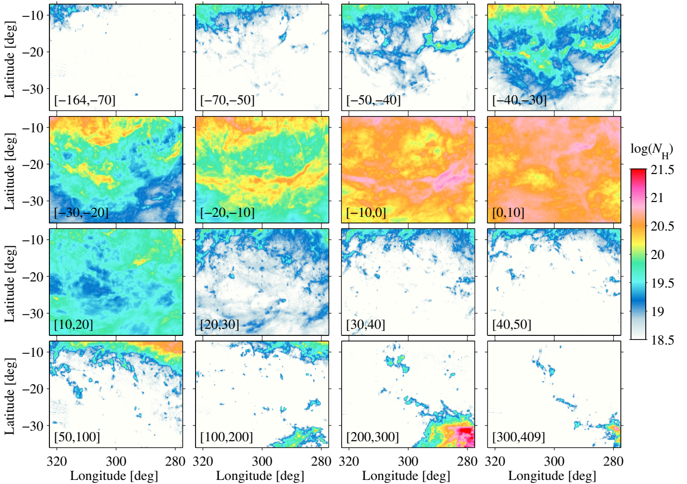
Fig. A.1. Maps of the N_{\text{H I}} column densities (in \text{cm}^{-2} ) obtained at 14.5 , resolution from the GASS survey for optically thin emission and integrated over contiguous velocity intervals between the values given in \text{km s}^{-1} on the lower left corner of each map.
