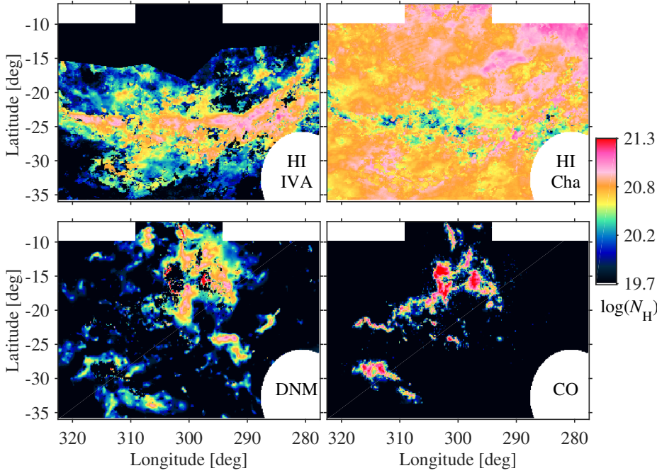
Fig. 15. N_{\text{H}} maps (in \text{cm}^{-2} ) for the different gas phases in the analysis region: H I in the intermediate velocity arc and, inside the Chamaeleon complex, gas in the H I, DNM, and CO-bright phases. The maps are based on the \gamma + A_{VQ} analysis, with the assumption of optically thin H I, the value of X_{\text{CO}\gamma} , and the dust DNM template calibrated in mass with the \gamma rays.
