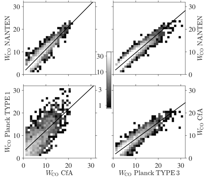
Fig. C.1. Correlations and linear regressions between the NANTEN, CfA, and Planck TYPE 3 and TYPE 1 W_{\text{CO}} intensities in the analysis region. The data are sampled at 0.125 and the intensities are given in \text{K km s}^{-1} . The best-fit slopes are given in Table C.1
