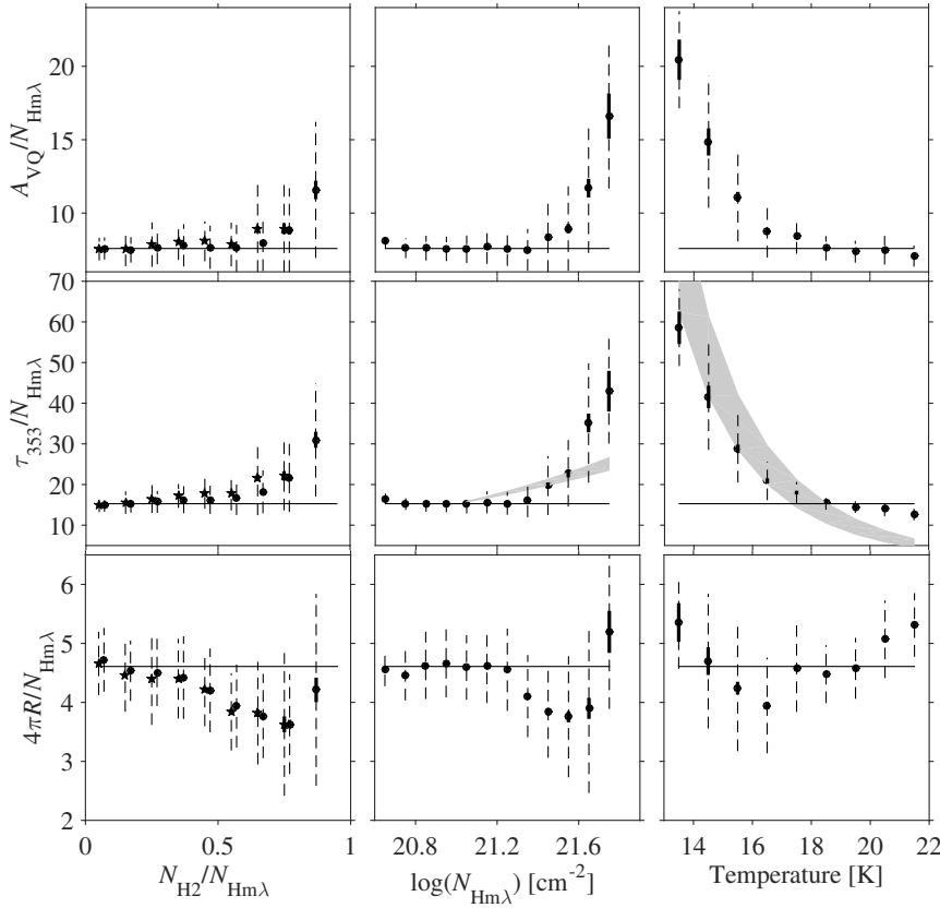
Fig. 13. Evolution of the dust properties per gas nucleon in intervals of molecular fraction in the gas column (left), of total gas column density N_{Hm\lambda} (middle), and of dust colour temperature (right). The A_{VQ}/N_H ratios are in units of 10^{-22} \text{ mag cm}^2 , \tau_{353}/N_H in 10^{-27} \text{ cm}^2 , and 4\pi R/N_H in 10^{-31} \text{ W} . To estimate the molecular fraction in N_H , we have assumed a DNM composition between half (stars) and fully (dots) molecular. The solid and dashed error bars respectively give the error on the means and the standard deviations in each sample. The thin lines mark the average values found in the (0.4-2) \times 10^{21} \text{ cm}^{-2} range. The shaded area in the temperature plot shows the expectation for uniform radiated powers ranging between 3.4 and 5 \times 10^{-31} \text{ W H}^{-1} , with the mean index \beta = 1.65 in the region. A power-law variation in opacity, \sigma_{353} \propto N_H^{0.28 \pm 0.03} , has been reported above 10^{21} \text{ cm}^{-2} in Orion. The shaded curve in the central plot shows this trend scaled at the value of the Chamaeleon complex opacity at N_{Hm\lambda} = 10^{21} \text{ cm}^{-2} .
