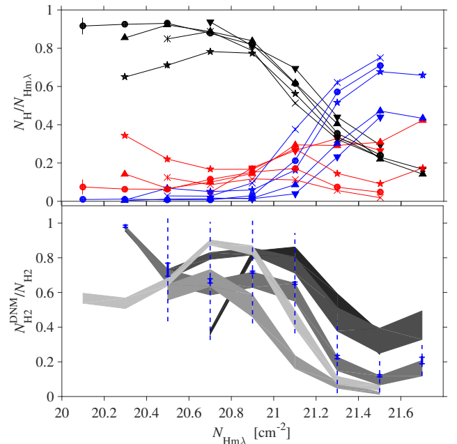
Fig. 16. Variations with N_{\text{H, Hm}\lambda} , in five separate clouds, of the fraction of the total column density in each phase (upper panel, H I in black, DNM in red, CO in blue) and of the fraction of the total \text{H}_2 column density that is CO dark (lower panel). Downward and upward triangles, stars, crosses, and circles refer to Musca, Cham I, Cham II+III, Cham East I, and Cham East II, respectively. The dark to light grey curves correspond to the clouds in the same order. The shaded areas cover the chosen uncertainty in DNM composition from 50% to 100% \text{H}_2 . The dotted and solid error bars give the standard deviations and errors on the mean in each N_{\text{H}} bin; they are shown for only one cloud and the fully molecular DNM case.
