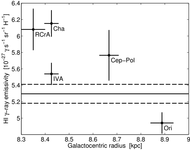
Fig. 7. Distribution, with Galactocentric radius, of the 0.4–10 GeV emissivities measured in the atomic gas of nearby clouds, for an H I spin temperature of 125 K. The \pm 1\sigma error bars are purely statistical. The solid line marks the mean emissivity measured within 1.5 kpc about the solar circle, for an H I spin temperature of 140 K. The dashed lines give the \pm 1\sigma error.
