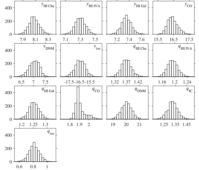
Fig. 4. Number distributions of the model coefficients obtained in the 1500 jackknife fits of the \gamma + A_{\text{VQ}} analysis for the optically thin H I case and overall energy band in \gamma rays. The y_{\text{H I},i} and y_{\text{DNM}} quantities are in units of 10^{-22} mag cm 2 , y_{\text{CO}} in 10^{-2} mag K -1 km -1 s, y_{\text{iso}} in 10^{-2} mag, q_{\text{CO}} in 10^{20} cm -2 K -1 km -1 s, and q_{\text{DNM}} in 10^{20} cm -2 mag -1 . The q_{\text{H I},i} , q_{\text{IC}} , and q_{\text{iso}} values are simple normalization factors.
