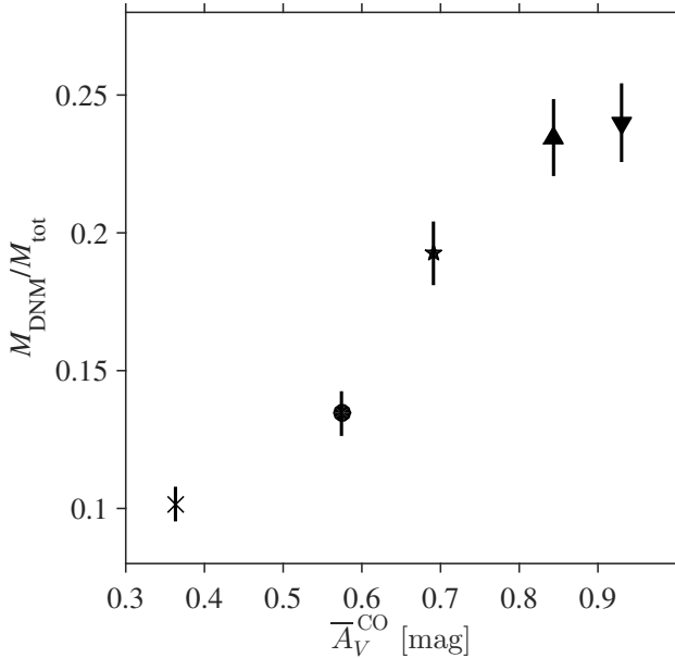
Fig. 18. Evolution of the DNM mass fraction with the average 2MASS extinction measured within the CO boundaries of each cloud. Downward and upward triangles, stars, crosses, and circles refer to Musca, Cham I, Cham II+III, Cham East I, and Cham East II, respectively.
