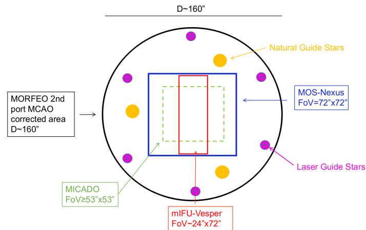
Figure 4. - The Field of View (FoV) of NEXUS (blue square, 1.2' \times 1.2' ) and the area probed by the IFs of VESPER (red rectangle, \sim 24'' \times 70'' ) are shown on the MORFEO 2nd port MCAO corrected area (black circle, diameter D \sim 160'' ). For comparison, the FoV of MICADO (green dashed square) is also shown. The purple filled circles represent the wavefront sensors for the 6 Laser Guide Stars used by MORFEO, while the yellow circles are those for the 3 Natural Guide Stars.
