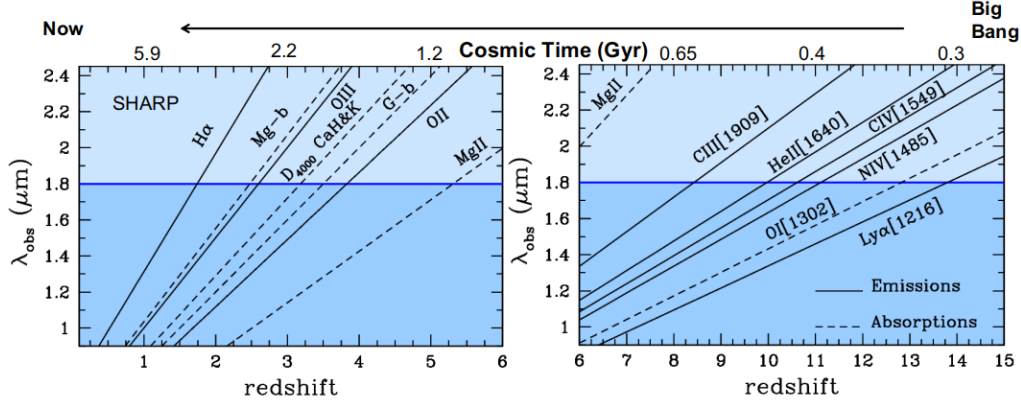
Figure 1. - The observed wavelength \lambda_{obs} = \lambda_{em} \times (1 + \text{redshift}) of the main nebular emission (black solid lines) and absorption (dashed lines) atomic lines are shown as a function of the redshift of the galaxy. The blue horizontal line marks the wavelength limit at \lambda = 1.8 \mu of the next generation spectrograph at ELT (MOSAIC and ANDES) and at VLT (MOONS).
