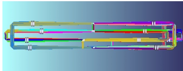
Figure 10. - Optical design of the Integral Field Selector system of one channel of VESPER. The 6 IFSs move along parallel planes to avoid vignetting.
