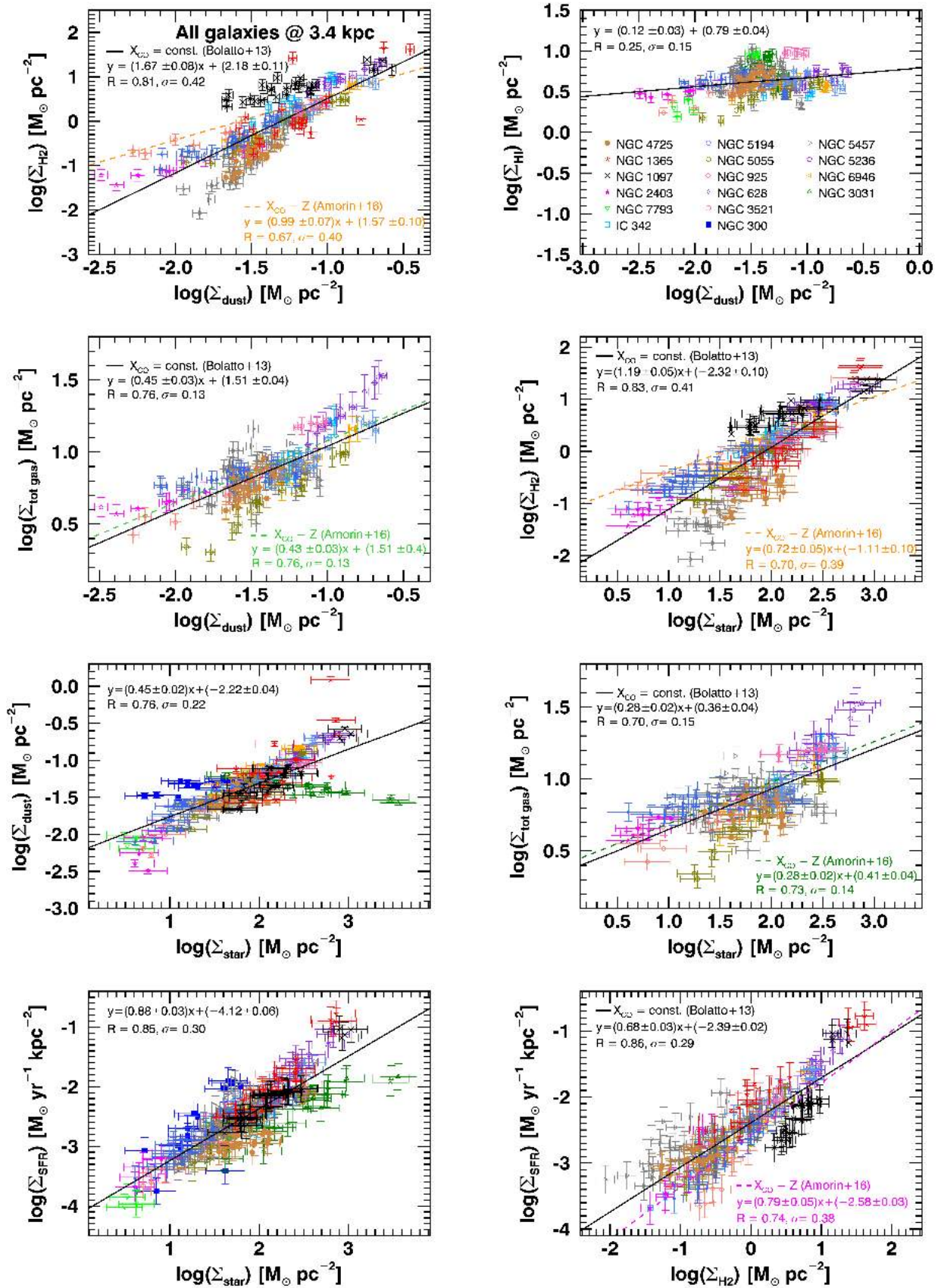
Fig. 2. Same as Fig. 1 for all sample galaxies evaluated together at the common scale of 3.4 kpc. Only data referring to the assumption of the constant X_{CO} are shown, while the drawn lines refer to the fits under the two assumptions on X_{CO} . Different symbols (and colors) represent different galaxies according to the legend shown in the panel displaying the \Sigma_{dust} – \Sigma_{HI} SR.
