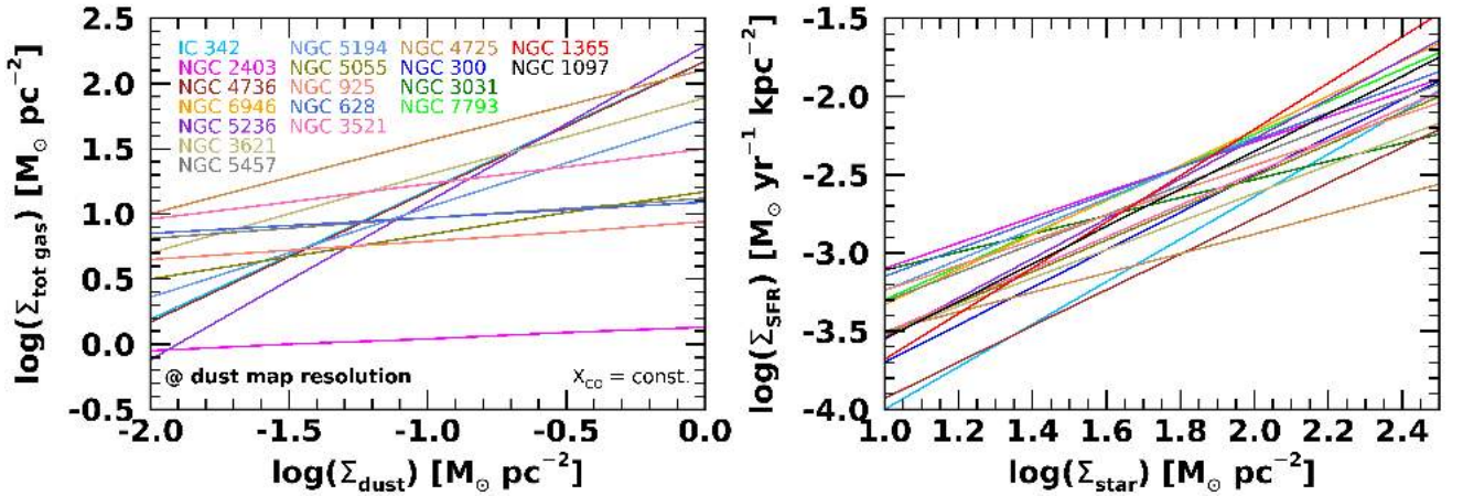
Fig. 3. Linear fits of the dust-total gas (left panel) and SFMS (right panel) SRs of sample galaxies individually evaluated at the physical scale imposed by the dust map resolution ( 36'' ), from 0.3 to 3.4 kpc (see Sect. 5.1). Each colored fit corresponds to a galaxy according to the legend shown in the left panel. The total gas refers to the assumption of the constant X_{\text{CO}} (Bolatto et al. 2013).
