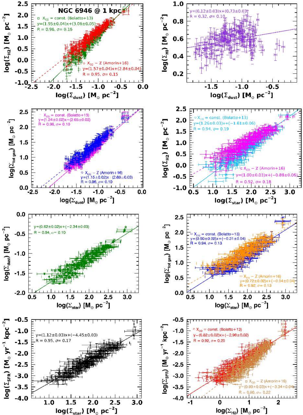
Fig. 1. Resolved SRs for the galaxy NGC 6946 within r_{25} at the resolution of 1 kpc, in logarithmic scale. From left to right: \Sigma_{\text{dust}}-\Sigma_{\text{H}_2} , \Sigma_{\text{dust}}-\Sigma_{\text{HI}} , \Sigma_{\text{dust}}-\Sigma_{\text{tot gas}} , \Sigma_{\text{star}}-\Sigma_{\text{H}_2} , \Sigma_{\text{star}}-\Sigma_{\text{dust}} , \Sigma_{\text{star}}-\Sigma_{\text{tot gas}} , \Sigma_{\text{star}}-\Sigma_{\text{SFR}} , \Sigma_{\text{H}_2}-\Sigma_{\text{SFR}} , \Sigma_{\text{tot gas}}-\Sigma_{\text{SFR}} , \Sigma_{\text{bar}}-\Sigma_{\text{SFR}} . Two sets of data are shown when the H 2 gas is involved according to the two assumptions on X_{\text{CO}} (see the legends). The lines are the linear fits to the data: continuum line for the constant X_{\text{CO}} (Bolatto et al. 2013), dashed line for the metallicity-dependent X_{\text{CO}} (Amorin et al. 2016). Fit parameters are also given in the figures.
