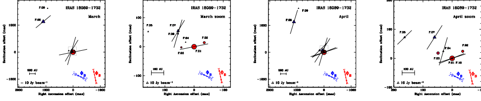
Figure 1. Masers identified in March (left) and April (right). The zoom is made on the region marked by the dashed grey boxes. Triangles and circles represent masers. The different sizes of the triangles and the circles represent the intensity. Line segments mark the direction of the polarisation angle for the maser features that show linear polarisation. The average direction of the resulting magnetic field \Phi_B obtained for two groups of masers is indicated in the bottom right corners of each panel.
