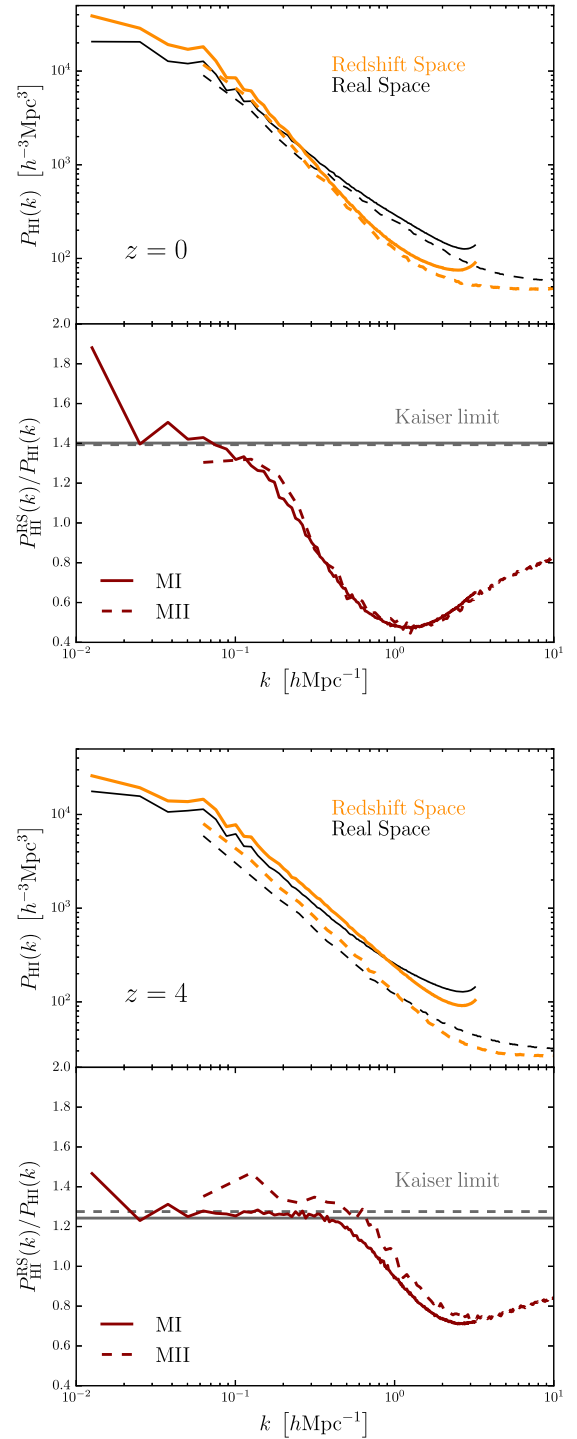
Figure 19. Comparison between the H I power spectrum computed in real space (black) and in redshift space (orange), for the MI (solid) and MII (dashed) simulations, for z = 0 (top) and z = 4 (bottom panels). In the lower sub-panel of each panel, we show the Kaiser limit for both the MI (grey solid) and the MII (grey dashed), computed as in equation (9), and compared to what is measured in simulations.
