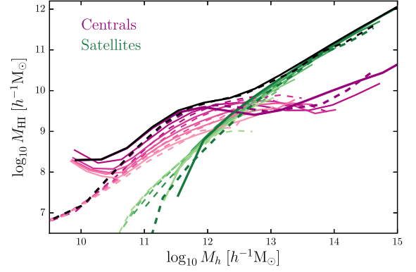
Figure 7. The median H I content of dark matter haloes for the MI (solid lines) and for the MII simulations (dashed lines) as a function of halo mass, for central galaxies (violet) and satellites (green). We report the results for redshift 0, 1, 2, 3, 4, and 5, with darker colours corresponding to lower redshifts. We show in black also the M_{\text{HI}}(M_h) obtained considering all galaxies at redshift z = 0 . At all redshifts, H I is found predominantly in satellite galaxies with halo masses M_h > 10^{12.5} h^{-1} M_\odot . For haloes of low and intermediate masses, instead, the dominant contribution comes from central galaxies.
