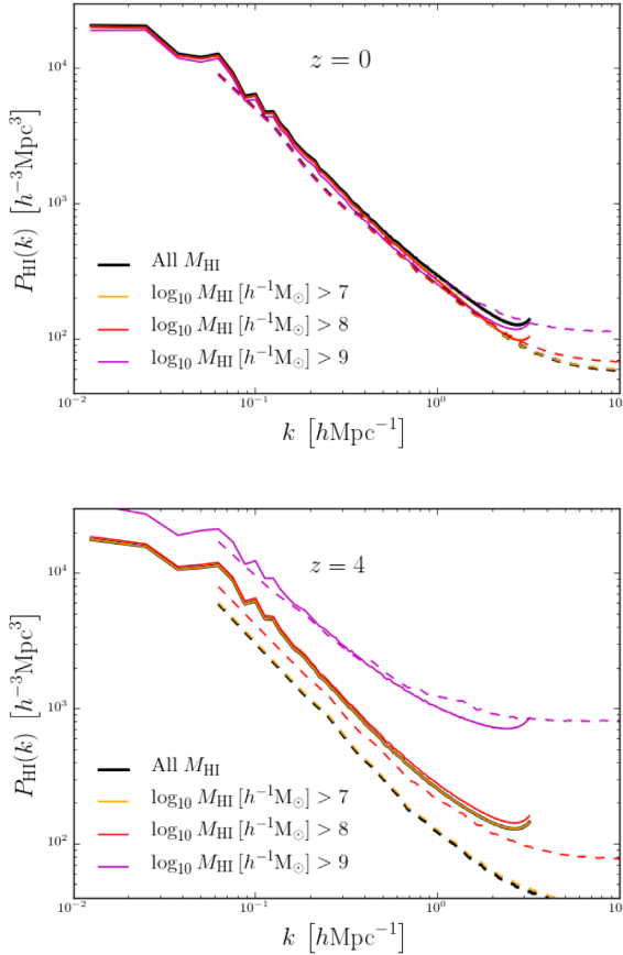
Figure 15. Top panel: The power spectrum of H I selected galaxies at z = 0 in the MI (solid) and MII (dashed lines) simulations, computed selecting galaxies with progressively larger H I mass. The total H I power spectrum (black) is the same as the one in Fig. 13. Bottom panel: Same as in the top panel, but at z = 4 .
