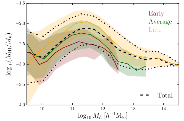
Figure 8. The ratio between the median H I halo mass function M_{\text{HI}}(M_h) and M_h for the MII simulation, at redshift z = 0 (black dashed), and its 16th and 84th percentiles (black dot-dashed lines). Red, green, and orange lines correspond to the same quantities computed for early, average, and late assembly haloes (see the text for definitions).
