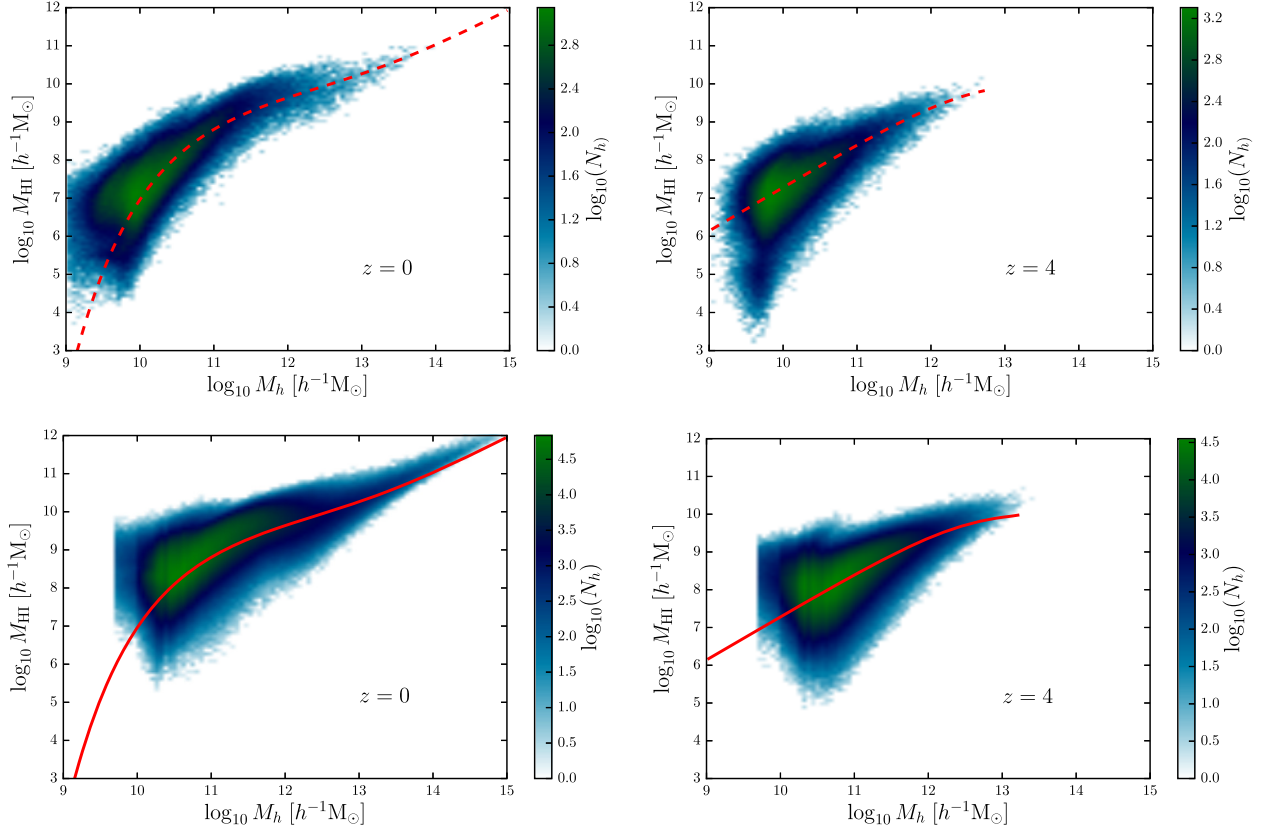
Figure B3. The predicted H I halo mass function M_{\text{HI}}(M_h) at redshift z=0 and redshift z=4 , colour coded by the number of haloes in each bin. The red lines show the best-fitting values of Table 2 obtained with the parametrization given in equation 2. Top panels: MII. Bottom panels: MI. Note that the best-fitting value reported here is the one from the MII case, to show the agreement between the two simulations.
