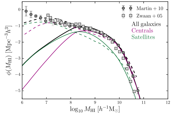
Figure 1. The H I mass function, i.e. the number density of galaxies with different H I mass, in the Millennium I (solid lines) and Millennium II (dashed lines) simulation at redshift zero. Magenta and green lines are used for centrals and satellites, respectively, while black lines are for all galaxies. Squares and circles with error bars show the data measured by Zwaan et al. (2005) and Martin et al. (2010) using the blind H I surveys HIPASS (Meyer et al. 2004, limited to z < 0.04 ) and ALFALFA (Giovanelli et al. 2005, limited to z < 0.06 ). In this work, we use M_s > 10^8 M_\odot for the MI and M_s > 10^6 M_\odot for the MII, as a compromise between resolution requirements and the inclusion of low H I mass galaxies in our sample.
