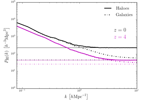
Figure 10. The real space power spectrum of galaxies (dot–dashed lines) for the MII simulation, weighted by their H I mass. Black lines and magenta lines are for z = 0 and z = 4 , respectively. At high k , this can be used to infer the level of shot noise and agrees, as expected, with the estimate that can be obtained using equation 4 (thin dot–dashed lines). We compare it with the ‘halo’ power spectrum at z = 0 (solid black) and z = 4 (solid magenta). We define ‘halo’ power spectrum the one computed considering all the H I content of galaxies at the centre of their hosting halo. The information on the spatial distribution of galaxies inside the halo is thus collapsed on to the central galaxy and the halo power spectrum flattens at larger scales. The shot noise associated with ‘haloes’ can be estimated from the power spectrum at small scales or using equation (4) (thin solid lines).
