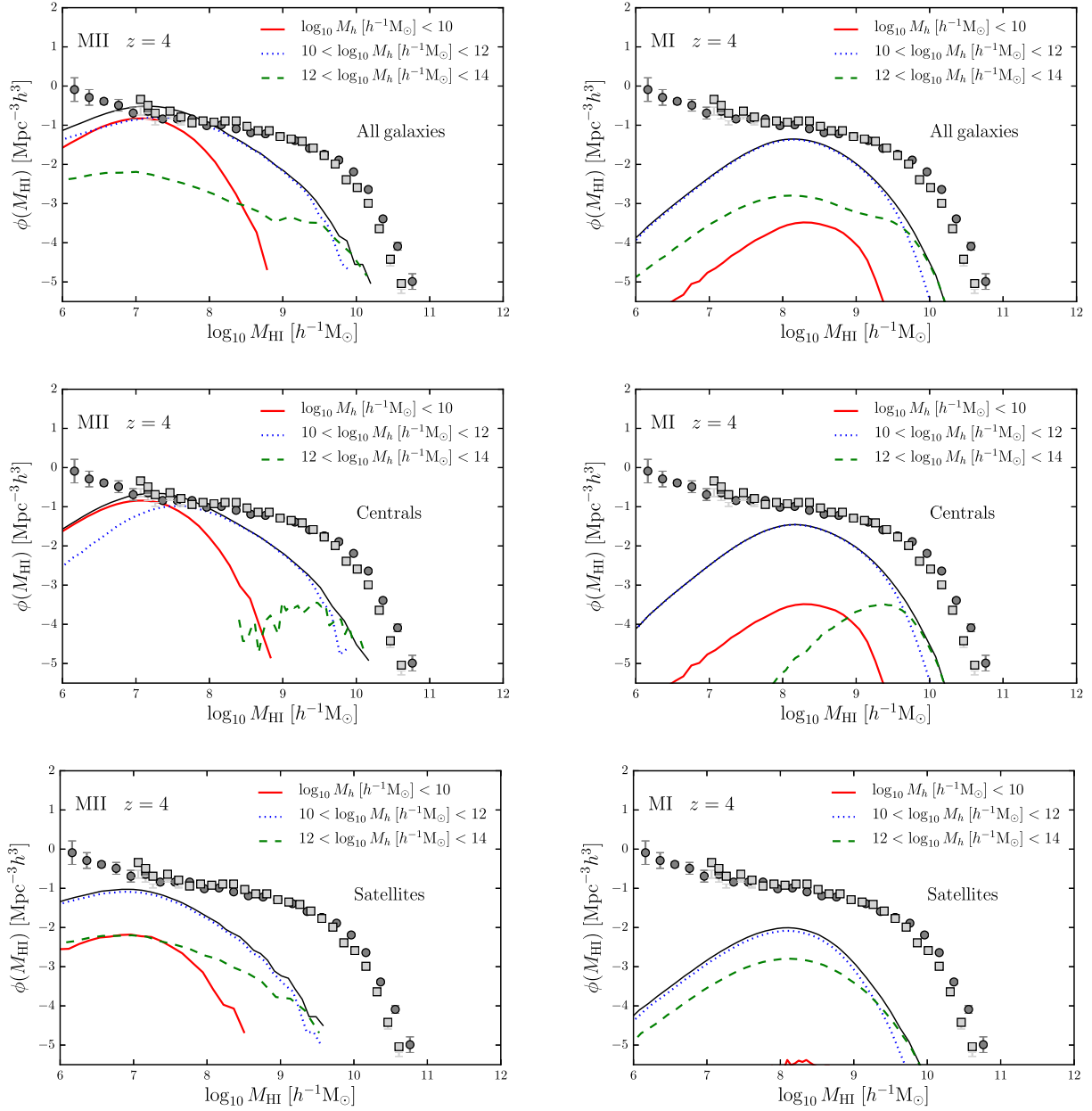
Figure A1. The predicted H I conditional mass function for the MII (left column) and the MI (right column) at z = 4 . In the middle and bottom panels, we separate the contribution from central and satellite galaxies, respectively. The solid black line in each panel is the sum of the contributions from different host dark matter haloes. To better appreciate the difference with z = 0 , we add with squares and circles the data measured by Zwaan et al. (2005) and Martin et al. (2010), the blind H I surveys HIPASS (Meyer et al. 2004) and ALFALFA (Giovanelli et al. 2005) in the local Universe.
