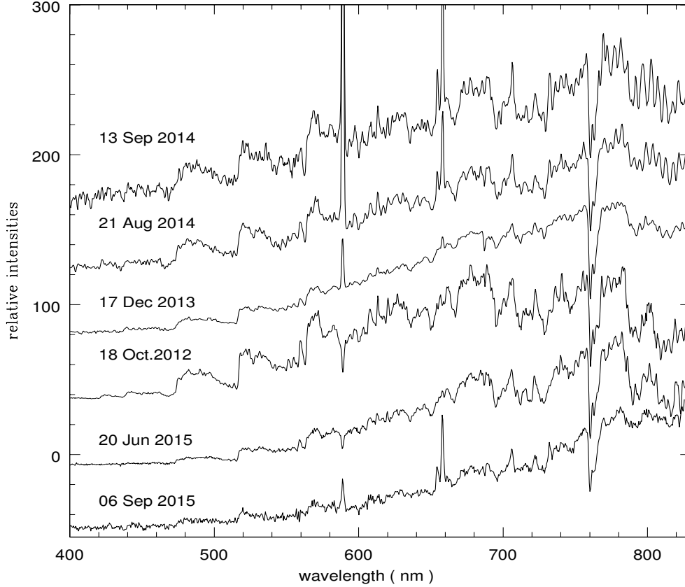
Figure 3. Optical spectra of V381 Lac taken between 2012 and 2015. The y axis represents relative intensities corrected for the atmospheric extinction. The spectra are normalise at 7800 Å. To allow for a better reading the 2013 and 2014 spectra are shifted upward with respect to the 2012 one; the 2015 spectra are placed at the bottom of the figure.
