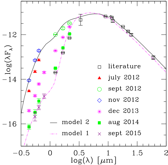
Figure 6. Spectral energy distribution of V381 Lac. Fluxes are in SI units. The literature data are from 2MASS, AKARI, IRAS, and WISE catalogs. The best fit models (see section 4 for the maximum (magenta dashed line) and minimum (black solid line) obscuration phases) are over imposed.
