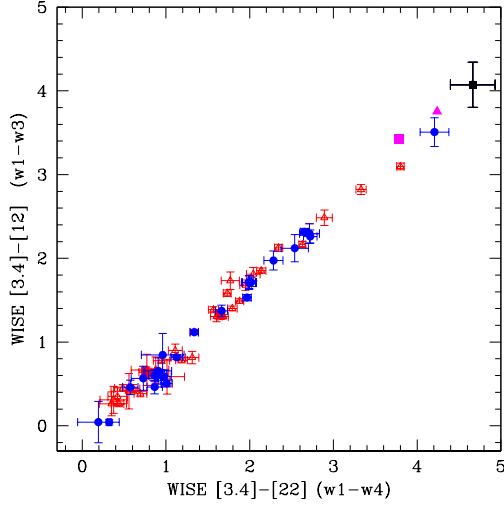
Figure 5. WISE w1-w3 vs w1-w4 colour colour diagram for the sample of carbon stars reported in the text. V381 Lac is the uppermost black square. Theoretical model 1 (magenta square) and model 2 (magenta triangle) are also over imposed.
