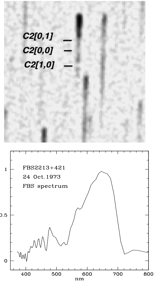
Figure 1. Top: two dimensional section of the FBS plate No 932. The digitization of V381 Lac shows a strong red head and allowed to identify the deep absorption bands of the C 2 from top to bottom at 5636, 5165, 4737Å, respectively. Bottom: wavelength calibrated spectrum; the central deep depression is partly due to the lower sensitivity of the plate emulsion.
