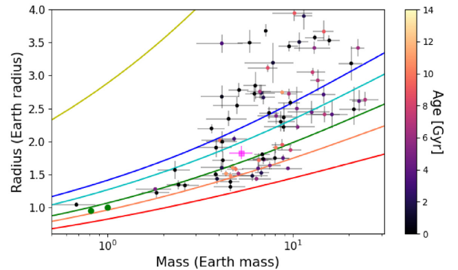
Figure 8. Mass–radius diagram of all planets smaller than 4 R_\oplus with a mass measurement significance better than 3\sigma (using data from the NASA exoplanet archive accessed 2020 June 11). The points are colour-coded according to their stellar host ages (in case no age was determined, the point is black). The green dots bottom left represent Venus and Earth, respectively. The solid lines show planetary interior models for different compositions, top to bottom: Cold H_2/He , 100 per cent H_2O , 50 per cent H_2O , 100 per cent MgSiO_3 , 50 per cent Fe, and 100 per cent Fe. The larger magenta square represents K2-111 b.
