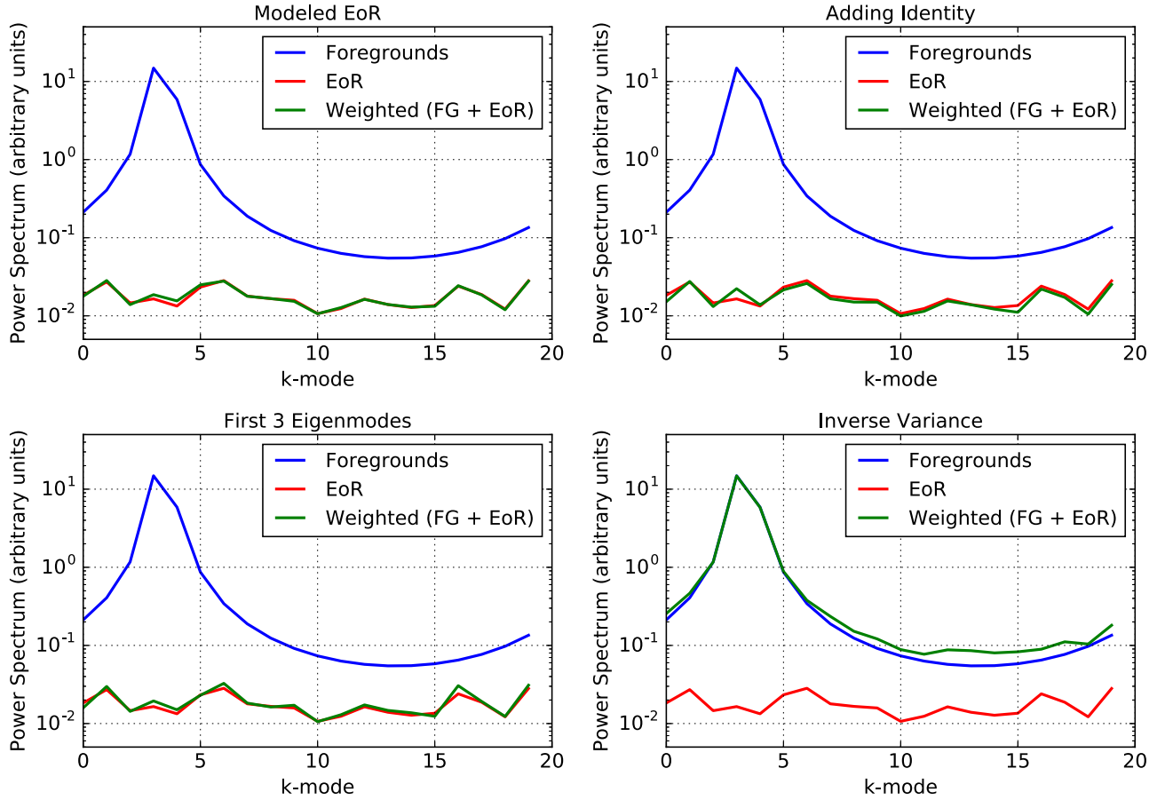
Figure 8. Resulting power spectrum estimates for our “fringe-rate filtered” (time-averaged) toy model simulation—foregrounds only (blue), EoR only (red), and weighted FG + EoR data set (green). We show four alternate weighting options that each minimize signal loss, including modeling the covariance matrix of EoR (upper left), regularizing \hat{C} by adding an identity matrix to it (upper right), using only the first three eigenmodes of \hat{C} (lower left), and keeping only the diagonal elements of \hat{C} (lower right). The first case (upper left) is not feasible in practice, since we do not know C_{FG} and C_{EoR} like we do in the toy model.
