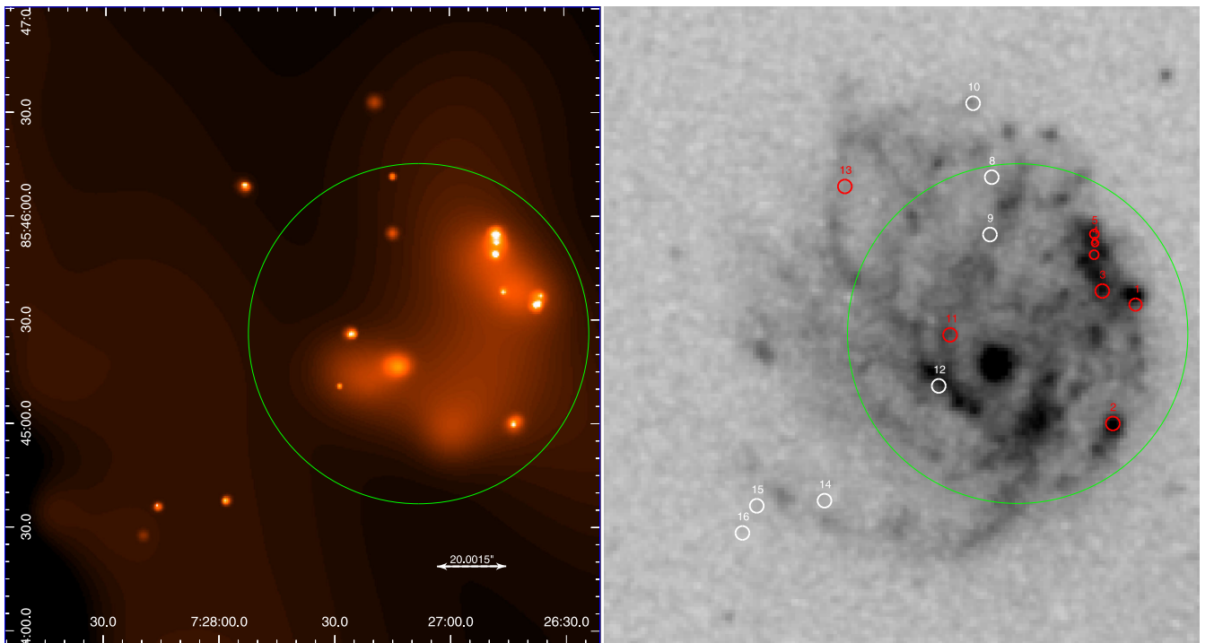
Figure 1. Left: smoothed image (csmooth) from Chandra data in the 0.5–7 keV band. The green circle (radius=50 arcsec) indicates the region used to extract the diffuse component spectrum (associated to S7, see the text for details). Right: the X-ray sources’ positions are overplotted on the optical image of NGC 2276 taken from the Digitized Sky Survey (DSS), see http://archive.stsci.edu/dss/index.html . Open circles and numbers identify detected point sources; red sources are ULXs. White sources have L_X^{0.5-10} \leq 10^{39} \text{ erg s}^{-1} .
