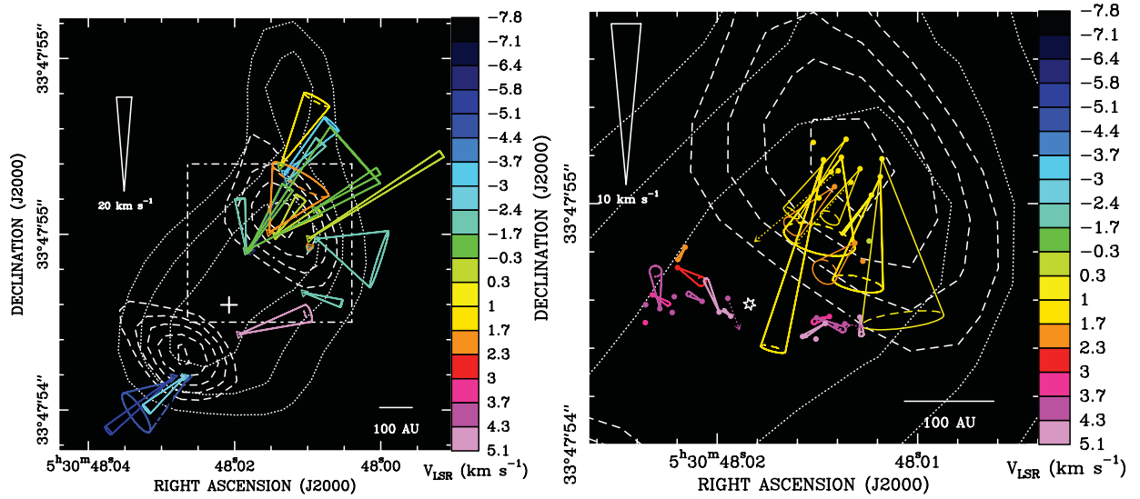
Figure 2. Proper motions of H 2 O ( left panel ) and CH 3 OH ( right panel ) masers in AFGL 5142 MM-1, as measured relative to their centers of motion, independently calculated for water ( cross ) and methanol ( star ). The rectangle in the left panel shows the area plotted in the right panel. The cones indicate orientation and uncertainties of measured proper motions (the amplitude scale is given in each panel) and colors denote l.o.s. velocities. Contour maps show the VLA 22 GHz (dotted line) and 8.4 GHz (dashed line) continuum.
