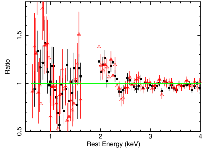
Figure 2. Data/model ratio in the soft X-ray energy region to the Suzaku data (XIS-FI: black filled squares; XIS1: red open triangles) and the model including the reflection component (modelled with PEXRAV). These residuals highlight the possible presence of an emission line at \sim 2.2 keV and of an absorption line at \sim 2.4 keV.
