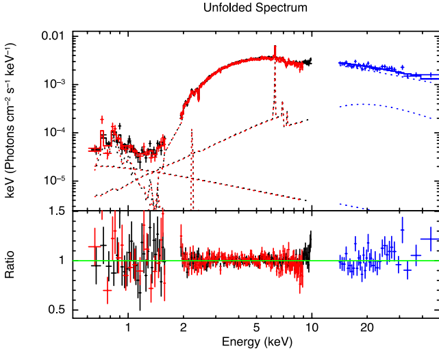
Figure 4. Suzaku 0.5–70 keV data and best-fitting model (XIS-FI: black; XIS1: red; HXD: blue) of Mrk 348; data have been rebinned for plotting purposes. The upper panel shows the data and best-fitting model described at the end of Section 3.1.2 (see Table 2 for the best-fitting parameters). The lower panel shows the data/model ratio to this model.
