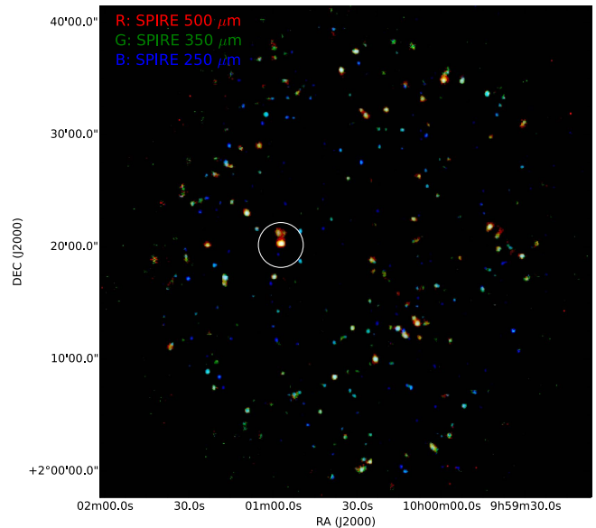
Figure 2. RGB Herschel /SPIRE composite color image of the COSMOS field covered by the CANDELS- Herschel survey. The R, G, and B channels correspond to SPIRE 500, 350, and 250 \mu\text{m} , respectively. Only sources brighter than 20 mJy at one or more of the three SPIRE wavelengths are shown. Sources with redder colors tend to be at higher redshifts. The large white circle with a radius of 2' indicates the position of the galaxy overdensity, which is the brightest SPIRE source in the whole field.
