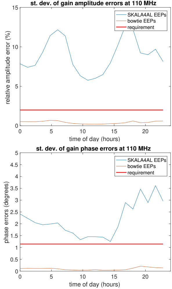
Fig. 3. RMS gain amplitude (top) and phase (bottom) estimation error across the array during a single day. The red line indicates the calibration accuracy requirement derived for the SKA-LOW stations [10].
