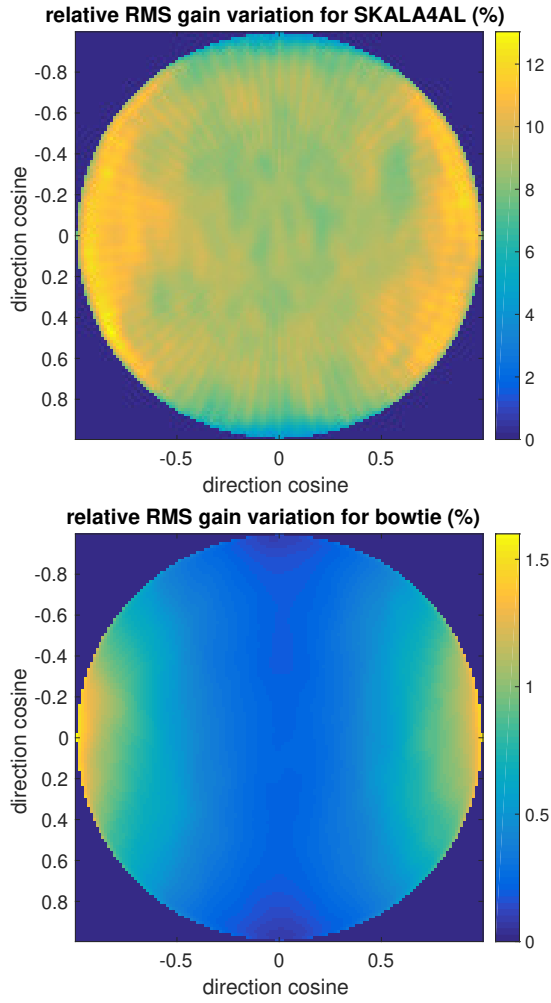
Fig. 2. RMS EEP gain variations across the entire visible sky expressed as percentage of the peak gain of the average EEP for a SKA-LOW station consisting of SKALA4AL antennas (top) or bowtie antennas (bottom).
