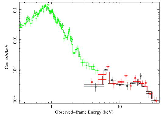
Figure 1. Chandra (green points) and NuSTAR FPMA and FPMB (black and red points, respectively) spectra of NGC 7130 and best-fitting modelling (see the text for details).
