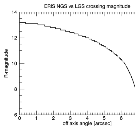
Figure 8 Transition magnitude vs NGS off-axis angle. Below the curve NGS-mode performs better than LGS-mode; the opposite above the curve.
