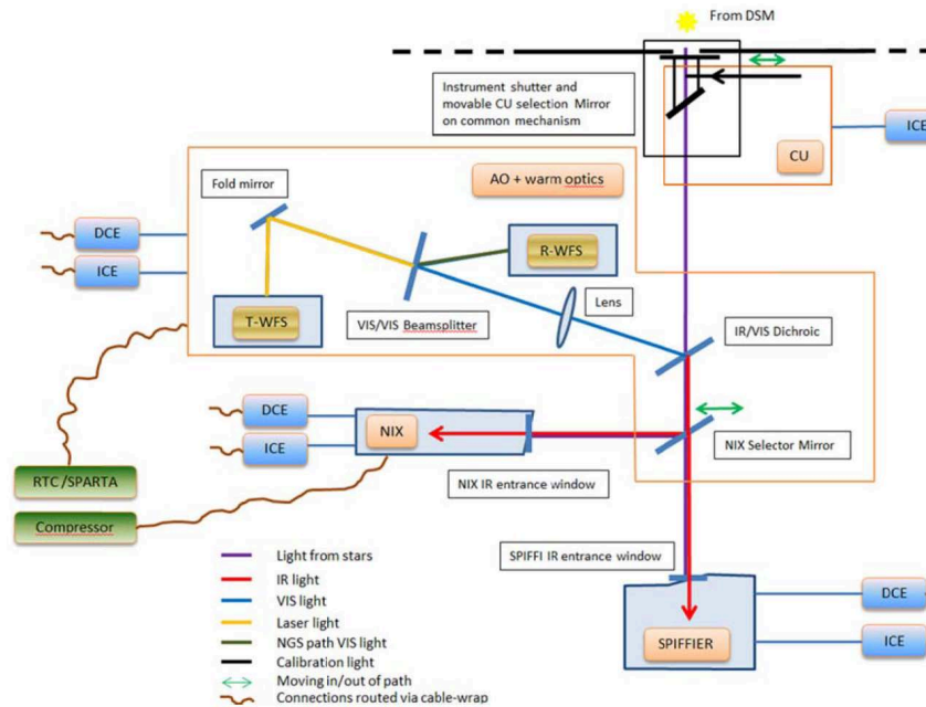
Figure 2 ERIS instrument scheme
