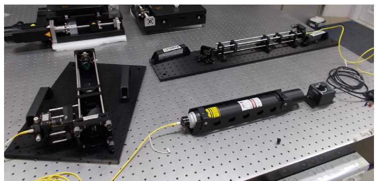
Figure 15 Alignment source for the NGS and LGS WFS
