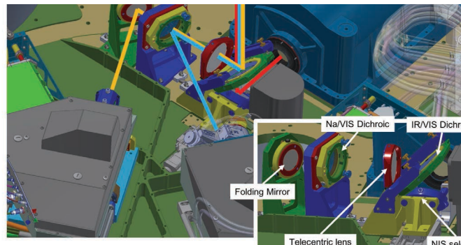
Figure 3. ERIS Warm Optics
