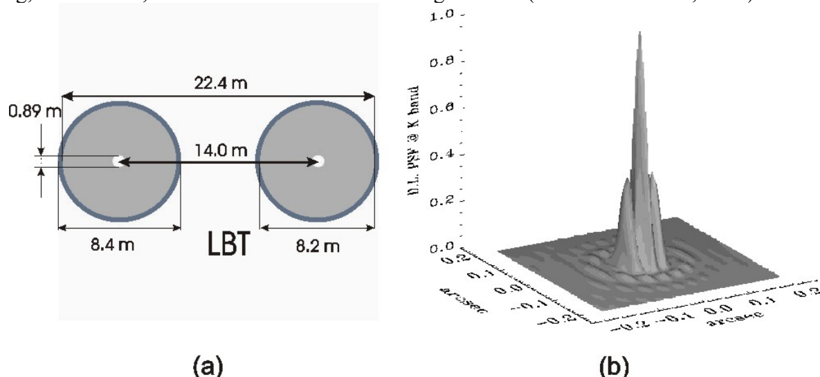
Figure 10 In the (a) picture are shown the specific dimension of LBT. The size of the primary seen by the secondary is 8.2 m instead of the overall 8.4 diameter. In (b) the interferometric diffraction limited PSF at K-band is shown.
