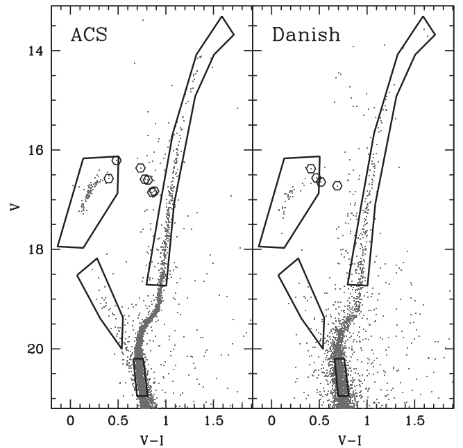
Figure 6. Zoomed view of the (V, V - I) ACS and ground-based CMDs. Selection boxes for MS, RGB, HB, and BSSs stars are shown. The RR Lyrae identified in the HB sample are marked with open hexagons.
