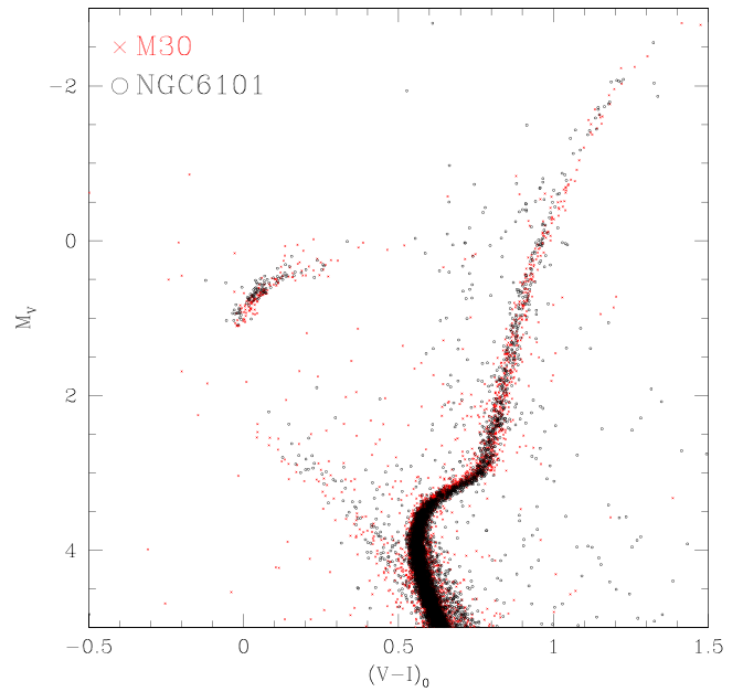
Figure 5. Superposition of the CMD of NGC 6101 (black open circles) to that of M30 (red crosses) in the absolute M_V , (V - I)_0 plane. For M30, we adopted the values of distance and extinction obtained by Ferraro et al. (2009). A distance modulus (m - M)_V = 16.20 \pm 0.1 and a color excess E(B - V) = 0.12 were then adopted for NGC 6101 to match the main evolutionary sequences of M30.
