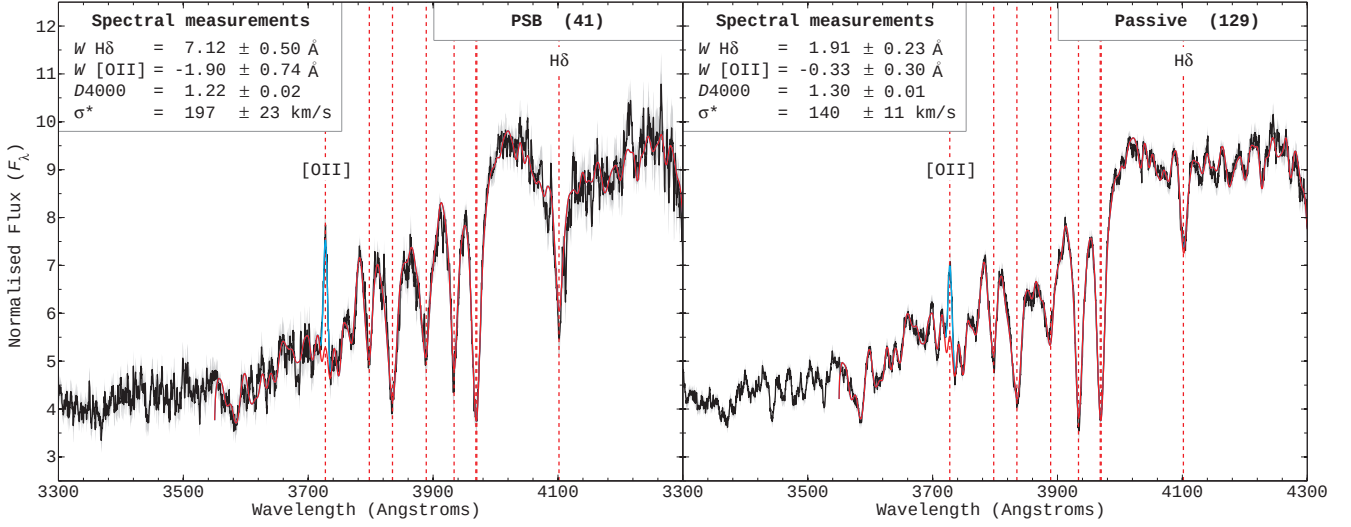
Figure 2. Red-optimised stacks: stacked optical spectra for our high redshift ( 1 < z < 1.4 ) PSB and passive galaxies, as determined from spectroscopic criteria (left-hand and right-hand panels, respectively). For these stacks, the individual rest-frame spectra were combined following a flux normalisation over the Balmer break region ( 3800 < \lambda_{\text{rest}} < 4170 \text{ \AA} ). Relevant sample sizes are shown in the legend, along with various spectral measurements (e.g. W_{\text{H}\delta} , W_{[\text{OII}]} , D_{4000} , \sigma_* ). Uncertainties in these spectral measurements ( 1\sigma ) are determined from the variance between measurements performed on 1000 simulated spectra generated via a bootstrap method. The errors in the stacked spectra (grey-shaded region) are 1\sigma confidence limits (see Section 2.3). In each case, a full spectral fit obtained from PPXF is shown for both the stellar component (red line) and the gas emission lines (cyan line).
