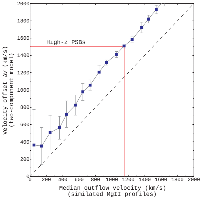
Figure A1. The calibration of our measured outflow velocities. A comparison of the typical (i.e. median) outflow velocity of our simulated Mg II profiles \tilde{v}_{\text{out}} with the velocity offset \Delta v returned by our two-component model. The data have been binned by the median outflow velocity \tilde{v}_{\text{out}} , and the error-bars represent the 1\sigma scatter in each bin. The dashed line shows the 1:1 relation. We find that for our two-component model, the outflowing component has a velocity offset \Delta v which systematically over-estimates the median outflow velocity \tilde{v}_{\text{out}} by \sim 350 \text{ km s}^{-1} . For our high- z PSBs, our two-component model yields an outflowing component with a velocity offset \Delta v \sim 1500 \pm 150 \text{ km s}^{-1} (red line). Therefore, these simulations suggest that the true outflow velocity is actually \tilde{v}_{\text{out}} \sim 1150 \pm 160 \text{ km s}^{-1} .
