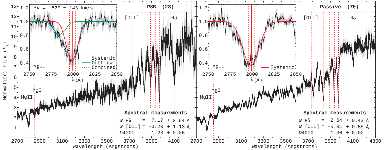
Figure 4. Blue-optimised stacks: stacked optical spectra for our high redshift ( 1 < z < 1.4 ) PSB and passive galaxies, as determined from spectroscopic criteria (left-hand and right-hand panels, respectively). For these stacks, the individual rest-frame spectra were combined following a flux normalisation over the Mg II continuum ( 2700 < \lambda_{\text{rest}} < 2900 \text{ \AA} ). Relevant sample sizes are shown in the legend, along with various spectral measurements (e.g. W_{\text{H}\delta} , W_{[\text{OII}]} , D_{4000} ). Uncertainties in these spectral measurements ( 1\sigma ) are determined from the variance between measurements performed on 1000 simulated spectra generated via a bootstrap method. The errors in the stacked spectra (grey-shaded region) are 1\sigma confidence limits (see Section 2.3). For each spectrum, the sub-panel shows the best fit to the Mg II absorption profile, using a model comprising two Gaussian-convolved doublets: one fixed at the systemic redshift (red line), and another with a free centroid to model the outflow (green line). The outflow component is only included in the model if required (as determined by an F-test). The rest-frame wavelengths of the Mg II doublet are also shown for reference (red-dashed lines). We find evidence for high-velocity outflows ( \Delta v \sim 1500 \pm 150 \text{ km s}^{-1} ) in our high- z PSBs, potentially representing the residual signature of a feedback process which quenched these galaxies. In contrast, we find no significant evidence for outflows in our high- z passive galaxies (the population our high- z PSBs will most likely evolve into).
