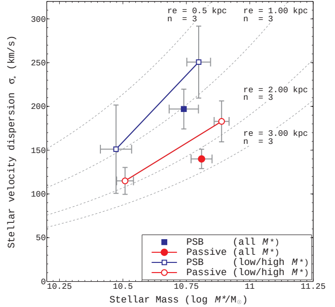
Figure 3. Stellar velocity dispersion \sigma_* as a function of stellar mass M_* for our high- z spectroscopically classified PSB and passive galaxies. Results are shown for both our full sample (filled symbols), and that separated by M_* (open symbols). In the latter, we separate our sample into low mass ( \log_{10} M_*/M_\odot < 10.7 ) and high mass ( \log_{10} M_*/M_\odot > 10.7 ). The \sigma_* measurements are plotted at the median M_* of the respective sample, with 1\sigma uncertainties determined from the variance between measurements performed on 1000 simulated spectra generated via a bootstrap method. Uncertainties in M_* ( 1\sigma ) are the standard errors in the median for the respective sample. As expected, \sigma_* increases with M_* for both populations. For high- z PSBs, there is a tentative indication that they present a higher \sigma_* than analogous passive galaxies, particularly at the highest masses ( M_* > 10^{10.7} M_\odot ). In this figure, we compare these results to the dynamical mass M_d(\sigma_*, r_e, n) relations, for various structural configurations (see Equation 4; dashed lines).
