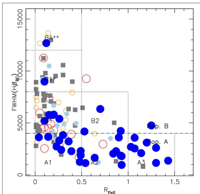
FIGURE 7 | Optical plane of 4DE1 as in Figure 6, for all low- z quasars with measurable HST/FOS UV spectra (Sulentic et al., 2007). Different symbols represent the amplitude of the CIV \lambda 1549 blueshift at half maximum c(\frac{1}{2}) normalized by FWHM(H \beta ) (a measure of the virial broadening): dark blue circles: \Delta v_r \leq -0.1 , pale blue: -0.1 < \Delta v_r \leq -0.05 ; gray (unshifted): -0.05 < \Delta v_r \leq +0.05 , pale red: km s ^{-1} +0.05 < \Delta v_r \leq +0.1 ; red: \Delta v_r \geq +0.1 . Filled symbols: Pop. A, open symbols: Pop. B, squares: RL, circles RQ.
