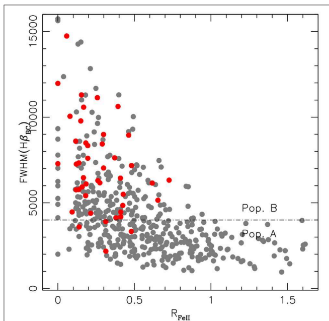
FIGURE 6 | The 4DE1 optical plane involving the width of H \beta and the strength of optical FeII. The horizontal line marks the boundary between population A (lower half of the diagram) and B (upper half) sources. Source occupation is shown for the 470 brightest SDSS-DR5 quasars ( z < 0.75 ) with highest S/N SDSS spectra (Zamfir et al., 2008). Gray and red dots represent RQ and lobe dominated LD RL quasars. The latter class shows a strong preference for the Population B zone.
