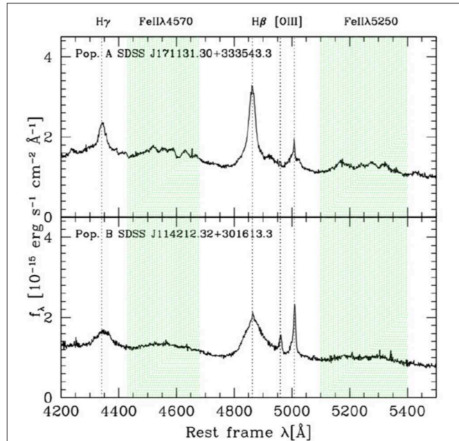
FIGURE 1 | The \text{H}\beta spectral range of two SDSS sources of Pop. A (top) and Pop. B (bottom). Abscissa is rest frame wavelength in Å, ordinate is specific flux in units of 10^{-15} \text{ erg s}^{-1} \text{ cm}^{-2} \text{ Å}^{-1} . The shaded areas indicate spectral regions where the main emission line contribution is due to Fe II opt . On the blue side of \text{H}\beta the wavelength range of the shaded area defines \text{FeII}\lambda 4570 i.e., the Fe II opt blended emission that is used to compute R_{\text{FeII}} and to characterize Fe II opt prominence along the quasar eigenvector-1 sequence.
