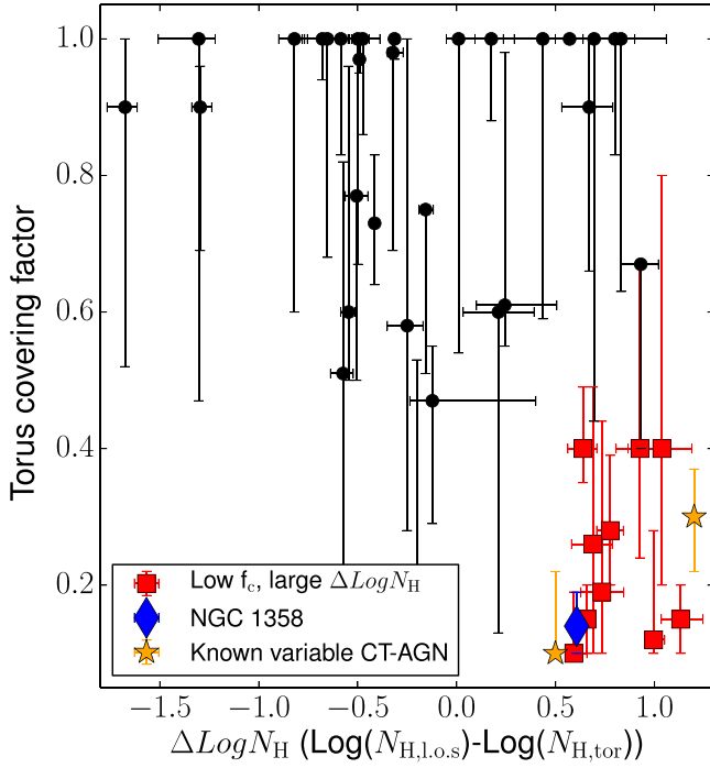
Figure 2. Obscuring material covering factor ( f_c ) as a function of the difference ( \Delta \text{Log} N_H ) between the logarithms of the LOS and torus average column density, for a sample of nearby CT-AGNs observed with NuSTAR and a 0.5–10 keV facility (XMM-Newton, Chandra, or Swift-XRT; from Marchesi et al. 2019; Torres-Albà et al. 2021). Sources with f_c < 0.4 and \Delta \text{Log} N_H > 0.5 are plotted as red squares. NGC 1358 is shown as a blue diamond: its large \Delta N_H and low f_c make it an excellent candidate clumpy environment CT-AGN. MRK 3 and NGC 4945, both known variable CT-AGN also having large \Delta N_H and low f_c , are plotted as orange stars.
