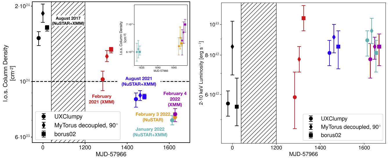
Figure 7. LOS column density (left) and 2–10 keV intrinsic luminosity (right) of NGC 1358 as obtained using UXCLUMPY (circles), MYTORUS decoupled in its 90° configuration (diamonds) and boru02 (squares) in each of the epochs where an X-ray observation was performed, starting from the joint NuSTAR–XMM–Newton observation taken in 2017 August. No luminosity variability was observed between the 2022 February 3 and 4 observations, so we plot only one data point. In the left panel, we show in an inset the results of the 2022 observations, to avoid overcrowding the plot. The UXCLUMPY and boru02 data points are shifted by 20 days (0.5 days in the N_{\text{H,LOS}} inset) for visualization purposes. To further increase the plot clarity, the first 1200 days (hatched area) are not in scale.
