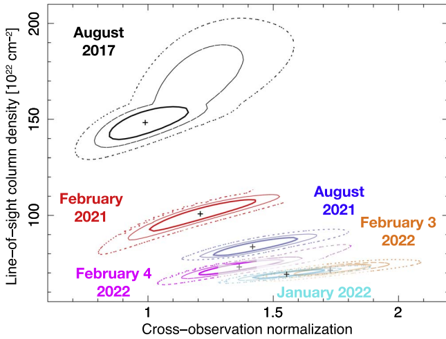
Figure 8. 68%, 90%, and 99% confidence contours of the LOS column density as measured using UXCLUMPY as a function of cross-observation flux normalization. In all contours, the cross-observation normalizations are the XMM–Newton ones: the only exception being the February 3 contours, which are computed using the NuSTAR normalization for consistency with the fact that N_{\text{H,LOS}} is also measured from the NuSTAR data alone. As discussed in the A4, the NuSTAR cross normalizations are usually \sim 10\% larger than the XMM–Newton ones.
