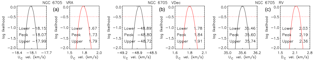
Figure 7. Likelihood of cluster properties for NGC 6705. Plots (a), (b) and (c) show the variation in log likelihood of the mean cluster velocity, U_c and the intrinsic cluster dispersion D_c for each velocity component. Text on the plots shows the peak and upper and lower 1\sigma probability values of the plotted parameter.
